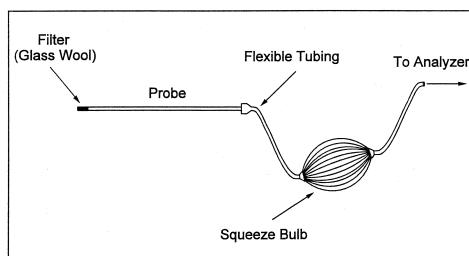
Figure 3-1. Grab-Sampling Train.
