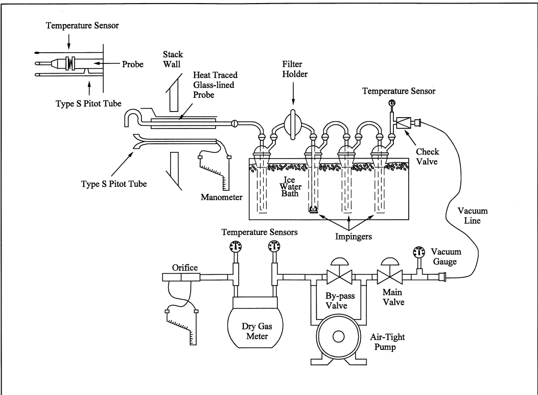
Figure 8-1. Sulfuric Acid Sampling Train.
