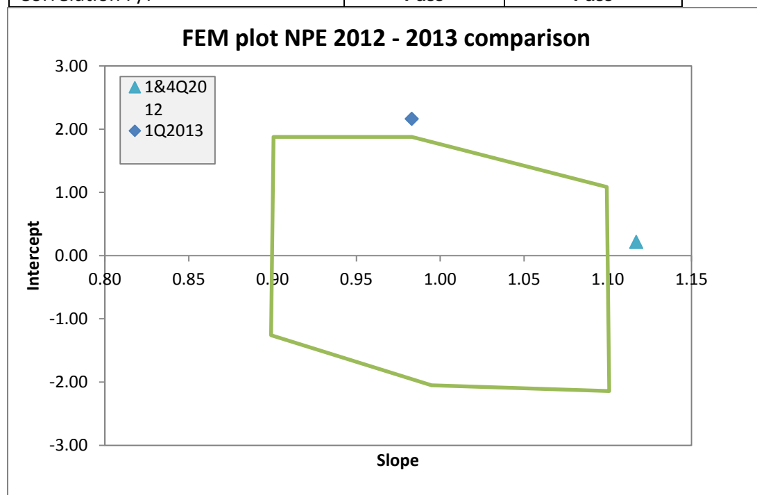
Figure 6. NPES FRM FEM Bias Plot; the green box represents the bounds of Class III performance criteria
