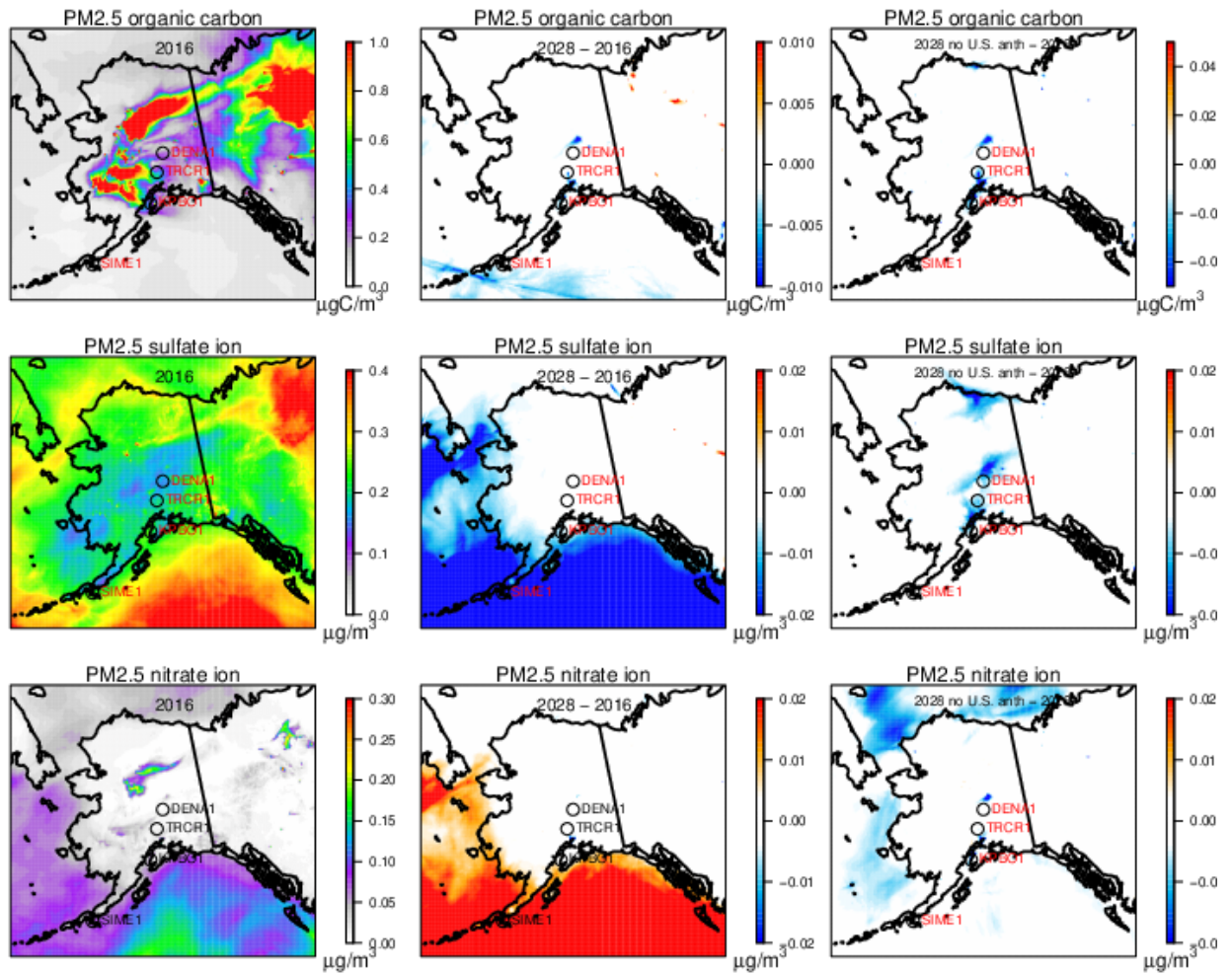
Figure A-3 Spatial plots showing the average model predictions for PM 2.5 organic carbon (top three panels), PM 2.5 sulfate ion (middle three panels), and PM 2.5 nitrate ion (bottom three panels) on the 20% worst days at Kenai Peninsula Borough.
