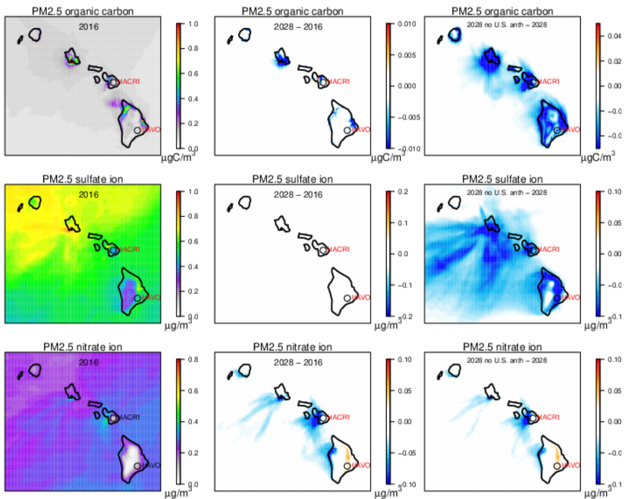
Figure B-1 Spatial plots showing the average model predictions for PM 2.5 organic carbon (top three panels), PM 2.5 sulfate ion (middle three panels), and PM 2.5 nitrate ion (bottom three panels) on the 20% worst days at Haleakala National Park. The left panels depict concentrations for year 2016, the middle panels depict the differences in concentrations for year 2028 – 2016, and the right panels depict the differences in concentrations for year 2028 with no anthropogenic influences minus year 2028.
