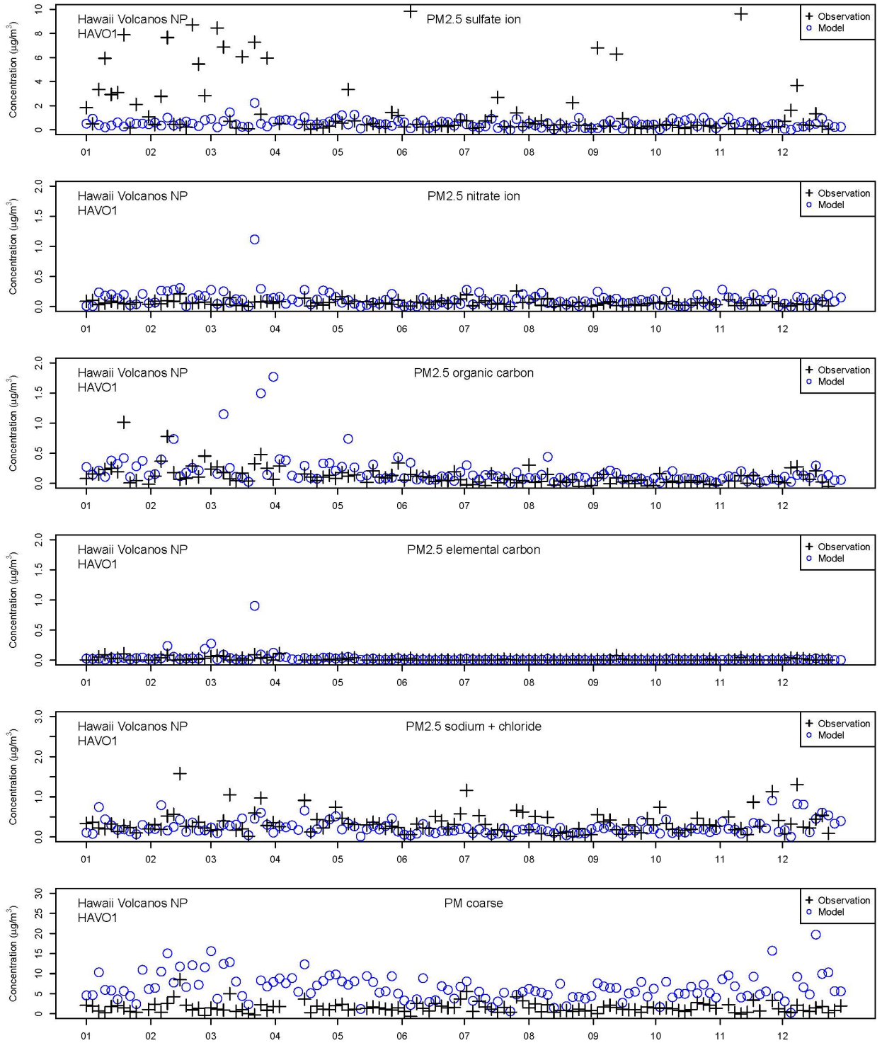
Figure B-4 Time series plots for 2016 comparing model predictions (blue circles) with IMPROVE monitor measurements (black crosses) for \text{PM}_{2.5} sulfate ion (top panel), \text{PM}_{2.5} nitrate ion (second panel), \text{PM}_{2.5} organic carbon (third panel), \text{PM}_{2.5} elemental carbon (fourth panel), NaCl (fifth panel), and PM coarse (bottom panel) at Hawaii Volcanoes National Park.
