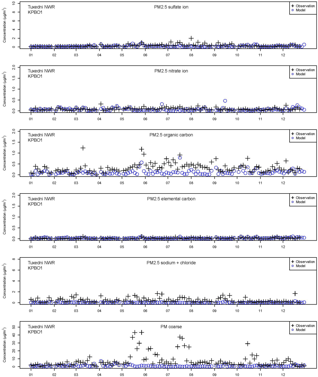
Figure A-7 Time series plots for 2016 comparing model predictions (blue circles) with IMPROVE monitor measurements (black crosses) for PM 2.5 sulfate ion (top panel), PM 2.5 nitrate ion (second panel), PM 2.5 organic carbon (third panel), PM 2.5 elemental carbon (fourth panel), NaCl (fifth panel), and PM coarse (bottom panel) at Kenai Peninsula Borough.
