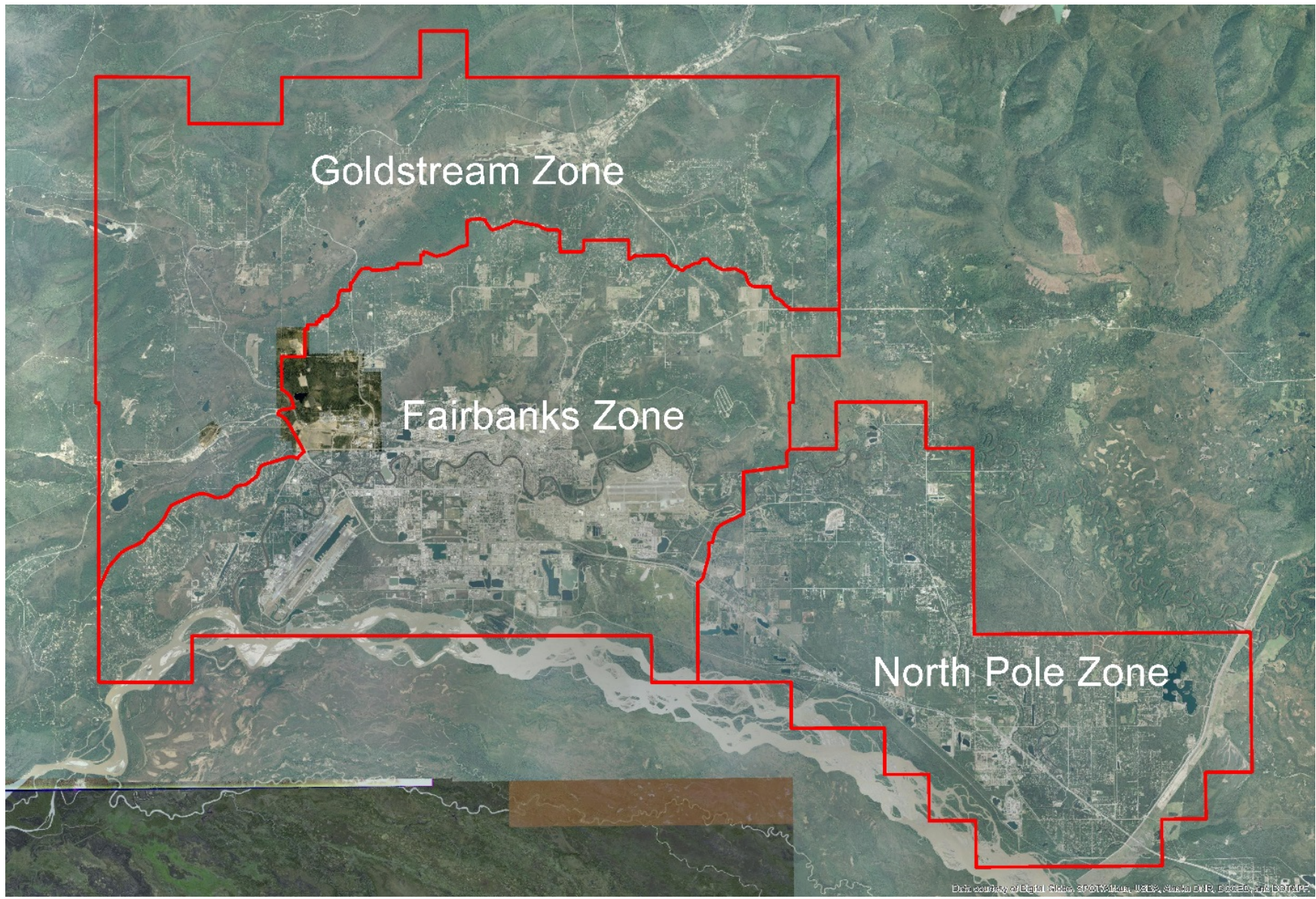
Figure 5.3-2. Air Quality Control Zones
