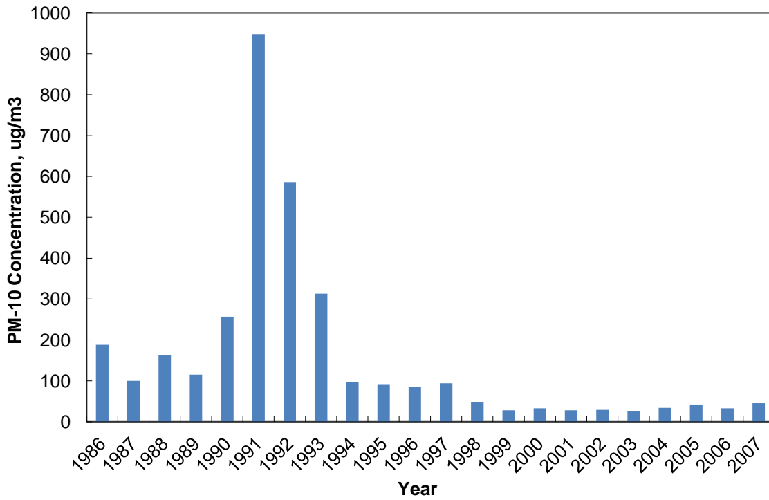
Juneau Maximum Daily PM-10 Concentrations
