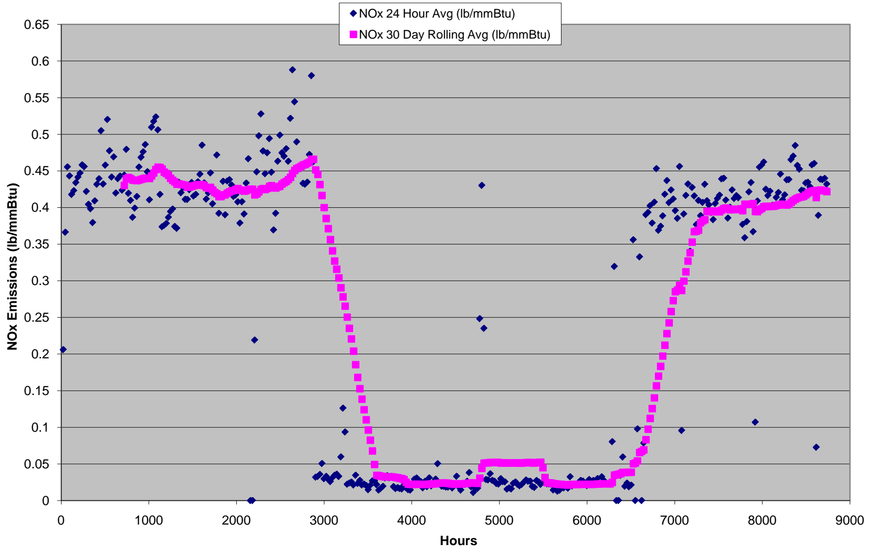
Chesapeake 3 '06 NOx Specific Emissions
