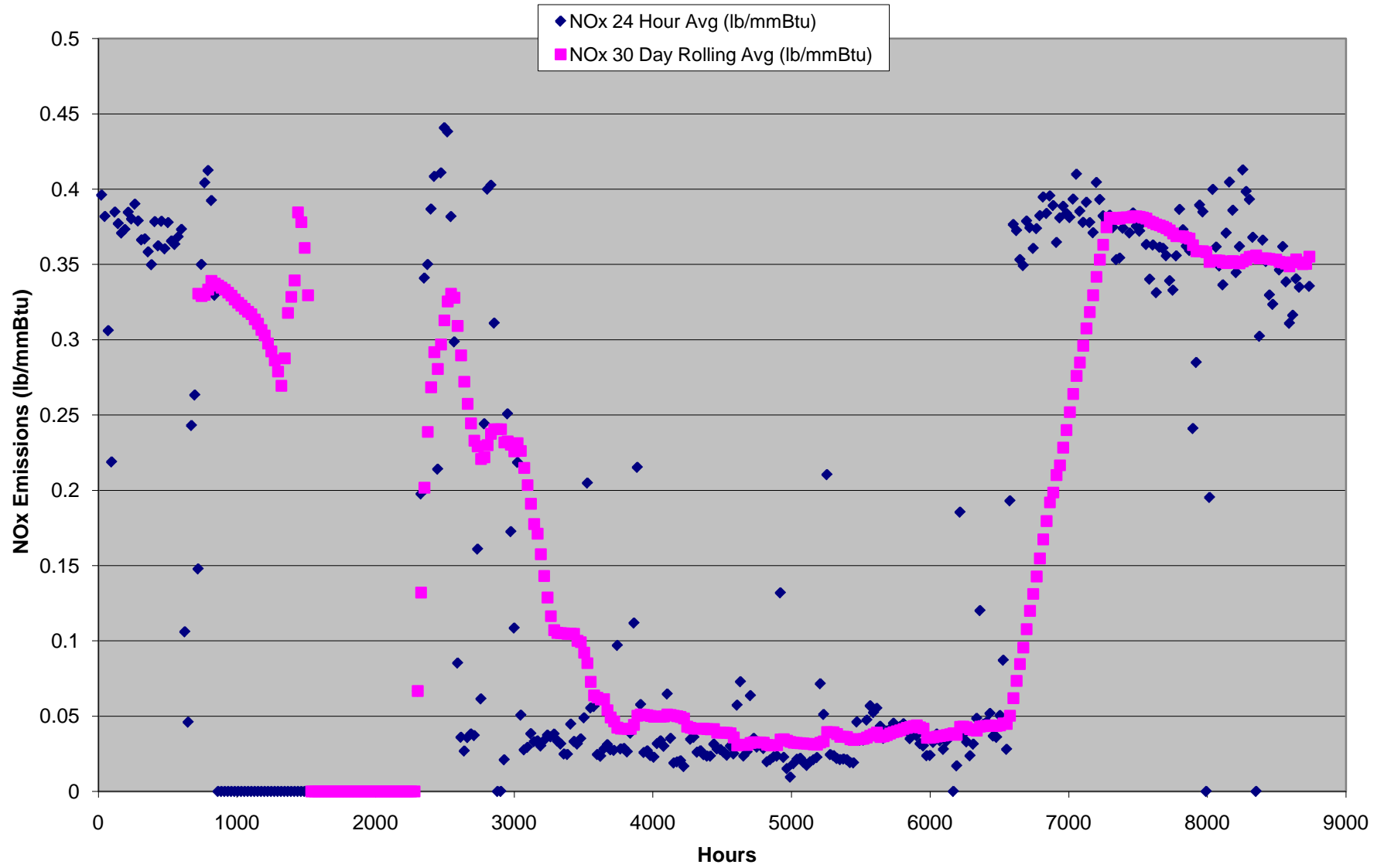
Mill Creek B4 '06 NOx Specific Emissions
