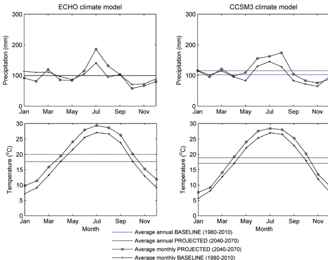
Figure 4. Average annual and monthly baseline (1980–2010) and projected (2040–2070) total precipitation and average temperature in McTier Creek Watershed for both (ECHAM4/HOPE-G [ECHO]) and Community Climate System Model, Ver 3 (CCSM3) climate change models under the A2 scenario of the Intergovernmental Panel on Climate Change Special Report on Emissions Scenarios. Average annual baseline and projected precipitation for the ECHO scenario are approximately identical; therefore, only 1 line is visible. [Color figure can be seen in the online version of this article, available at wileyonlinelibrary.com .]
