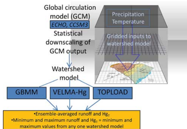
Figure 2. Conceptual modeling approach showing the input of statistically downscaled gridded climate change projections (ECHAM4/HOPE-G [ECHO]; and Community Climate System Model, Ver 3 [CCSM3]) to 3 separate watershed models (Grid-Based Mercury Model [GBMM], Visualizing Ecosystems for Land Management Assessment Model for Hg [VELMA-Hg], and the TOPography based constituent LOADING model [TOPLOAD]) to produce ensemble-averaged runoff and total mercury (THg) concentration and flux projections, in addition to minimum and maximum runoff, THg concentration, and THg flux projections. [Color figure can be seen in the online version of this article, available at wileyonlinelibrary.com .]
