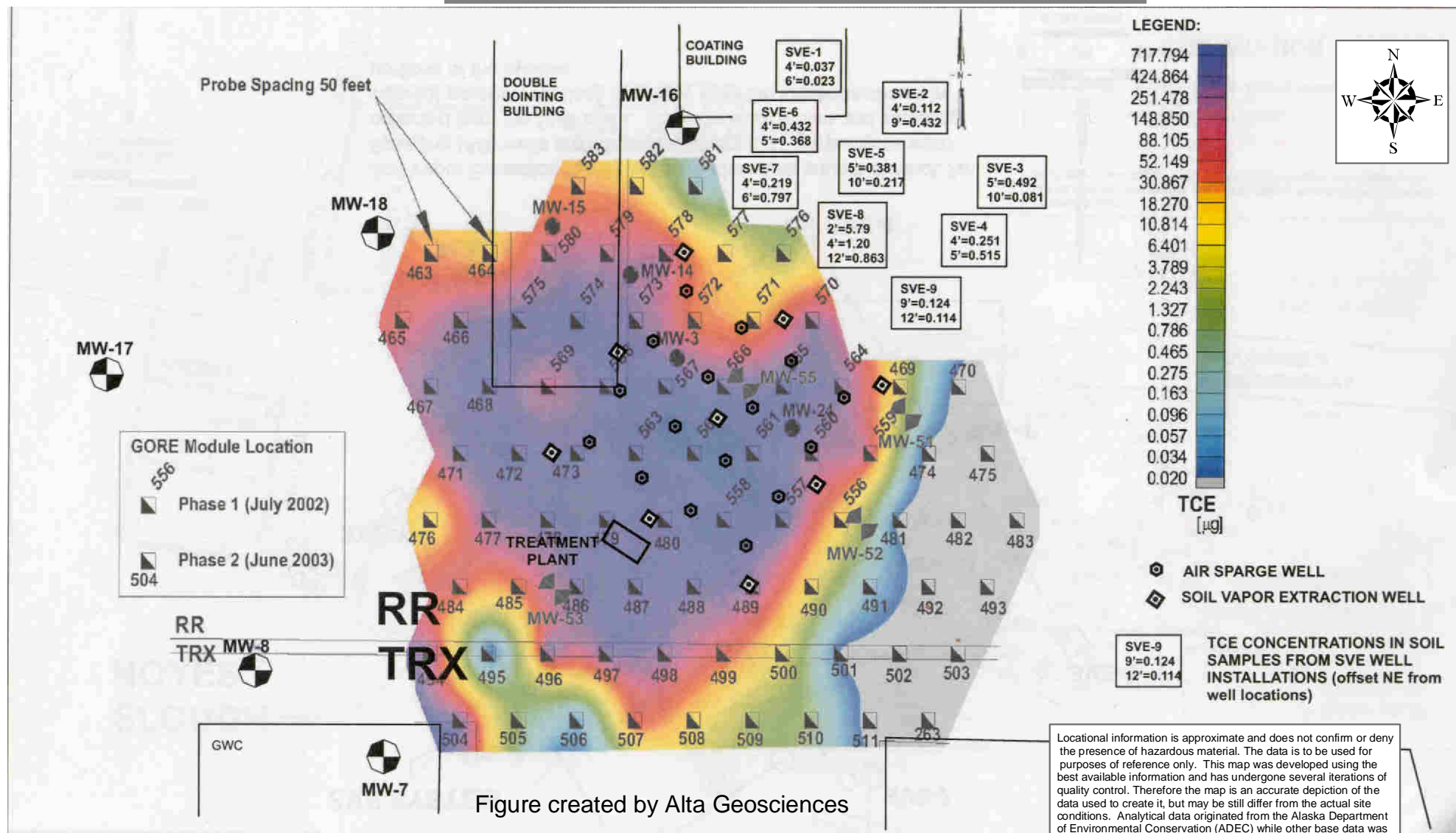
Figure 2 - TRICHLOROETHENE CONCENTRATIONS IN SOIL
