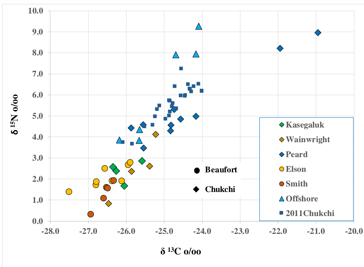
Figure 23. Biplot of \delta_{o/oo} for isotopes of carbon ( ^{13}\text{C} ) and nitrogen ( ^{15}\text{N} ) in estuaries and lagoons in the Chukchi and Beaufort Seas. Also plotted are the Wainwright offshore transect and isotope data from the coastal Chukchi Sea collected in 2011 (Dasher et al. 2016).
