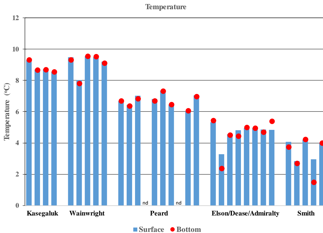
Figure 10. Surface and bottom water temperatures in estuaries and lagoons in the Chukchi and Beaufort Seas. (nd=no data)
