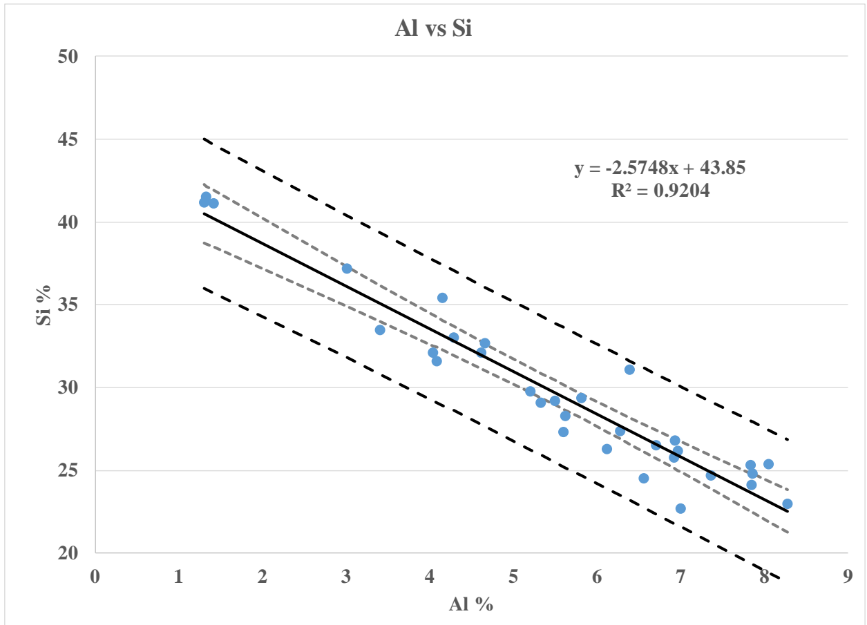
Figure 14. Relationship between sediment silicon and aluminum in estuaries and lagoons in the Chukchi and Beaufort Seas, including sample confidence limits (light dashed lines) and 99% prediction limits (heavy dashed lines).
