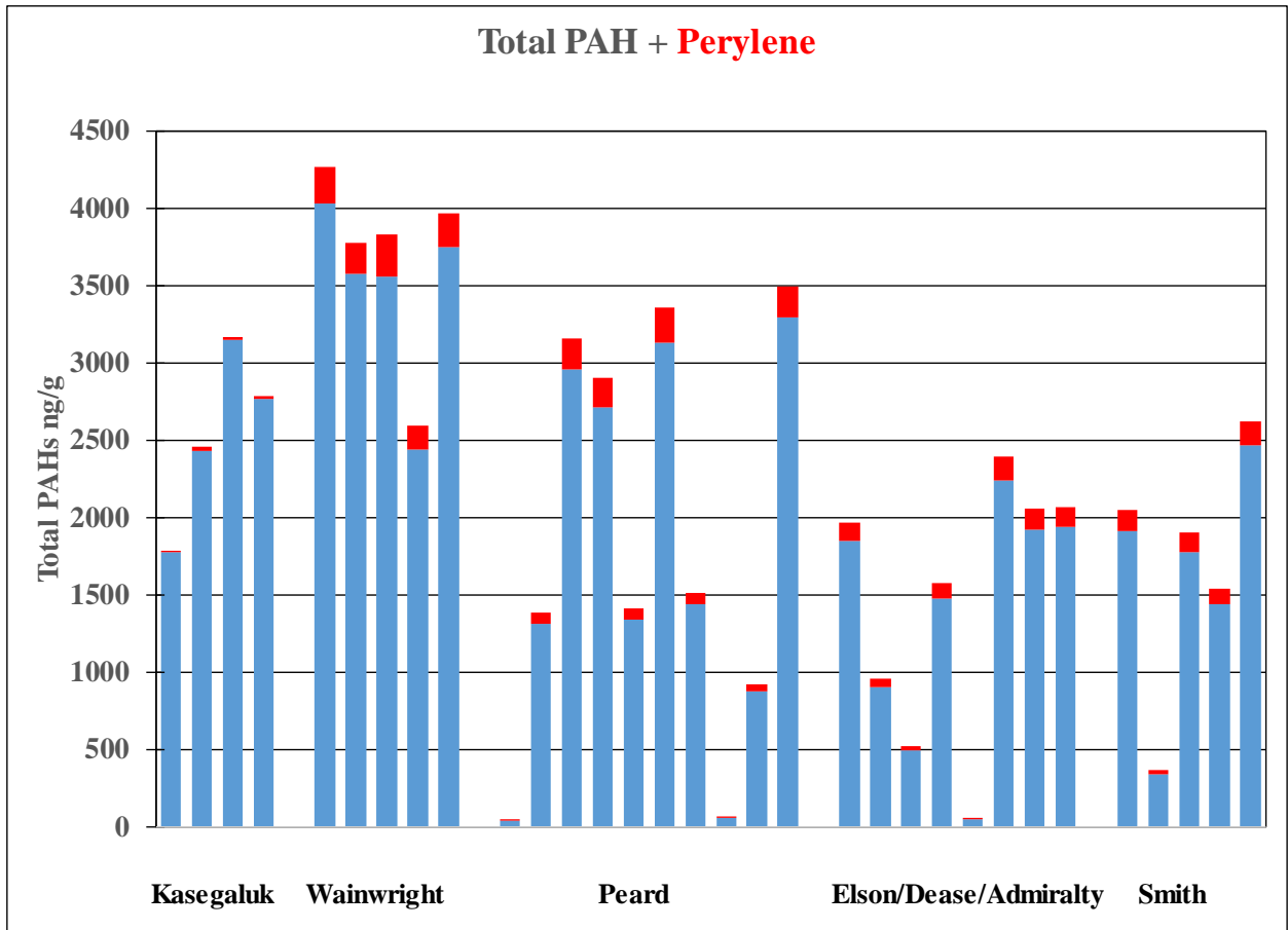
Figure 18. Total PAH concentrations with perylene (in red) in estuaries and lagoons in the Chukchi and Beaufort Seas.
