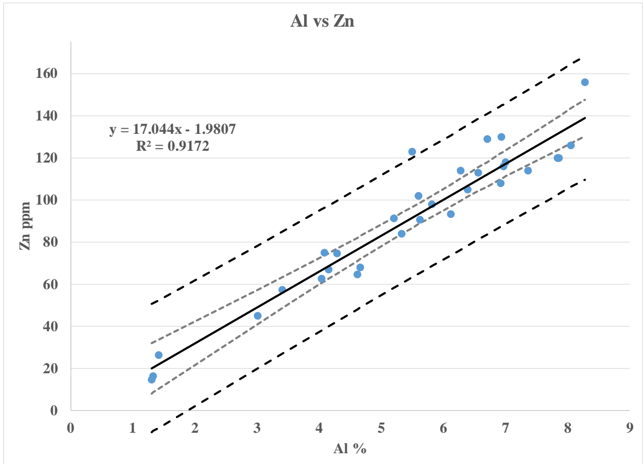
Figure 15. Relationship between sediment zinc and aluminum in estuaries and lagoons in the Chukchi and Beaufort Seas, including sample confidence limits (light dashed lines) and 99% prediction limits (heavy dashed lines).
