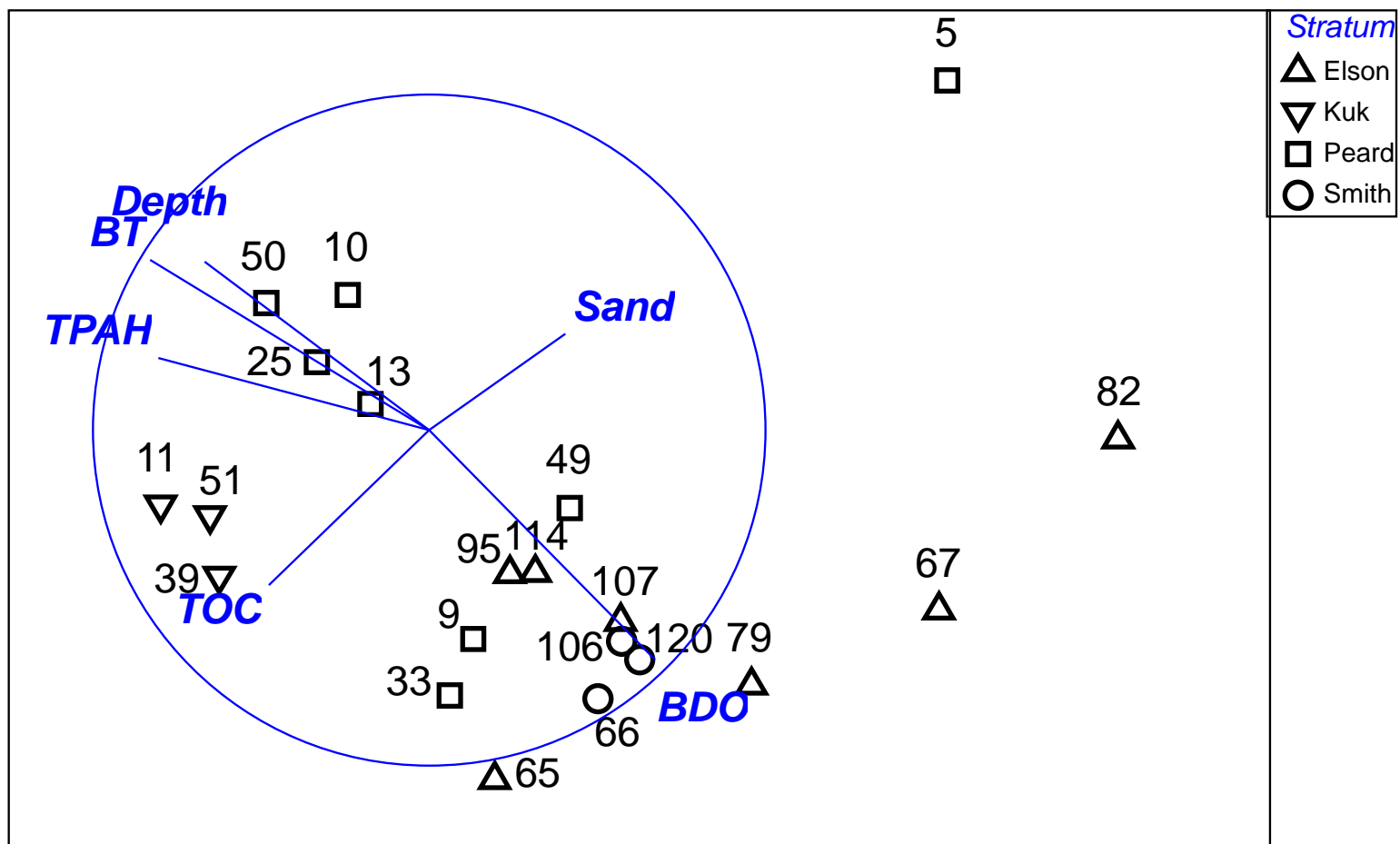
Figure 26. MDS ordination plot of Arctic estuaries based on physical variables at each station. (BT = bottom temperature, BDO = bottom dissolved oxygen, TOC = total organic carbon, TPAH = total PAHs).
