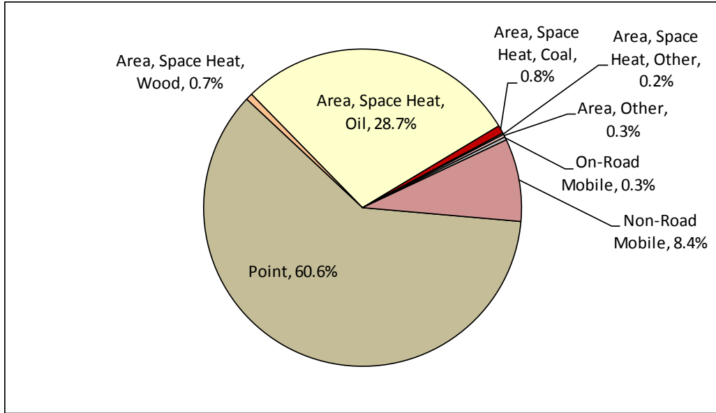
Figure 7.6-16. 2013 Baseline Episodic Nonattainment Area Emissions, Relative SO 2 Contributions (%)
