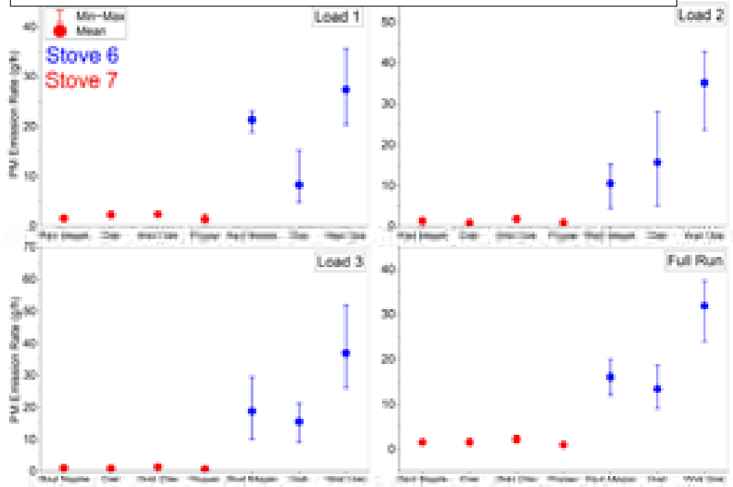
Figure 2. IDC comparison Stove 6 (Non-Catalytic) & Stove 7 (hybrid) – Grams per Kilogram
