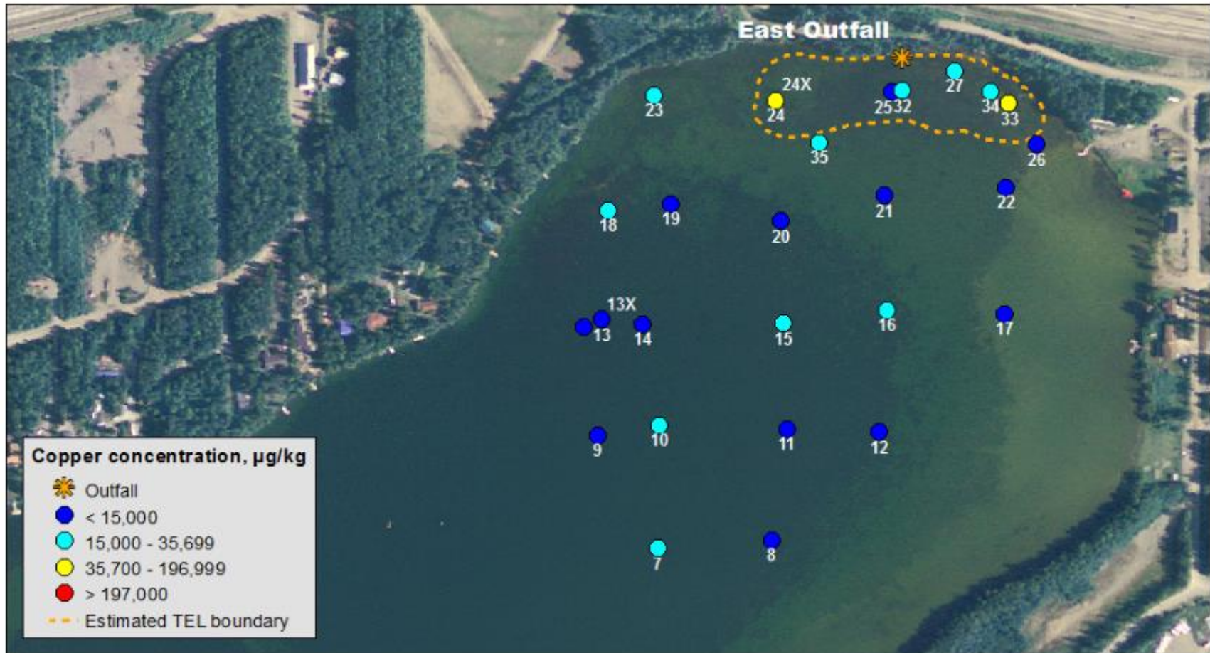
Figure 4. Distribution of bed sediment copper concentrations adjacent to the east outfall. Yellow markers indicate sites where concentrations exceed TEL values and red markers indicate sites that exceed PEL values. Dashed line is estimated area where copper concentrations are likely to exceed TEL values.
