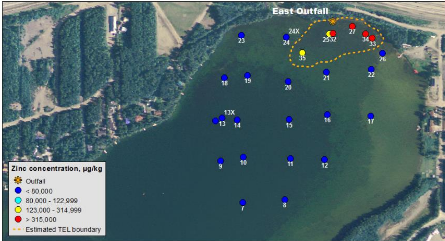
Figure 6. Distribution of bed sediment zinc concentrations adjacent to the east outfall. Yellow markers indicate sites where concentrations exceed TEL values and red markers indicate sites that exceed PEL values. Dashed line is estimated area where zinc concentrations are likely to exceed TEL values.
