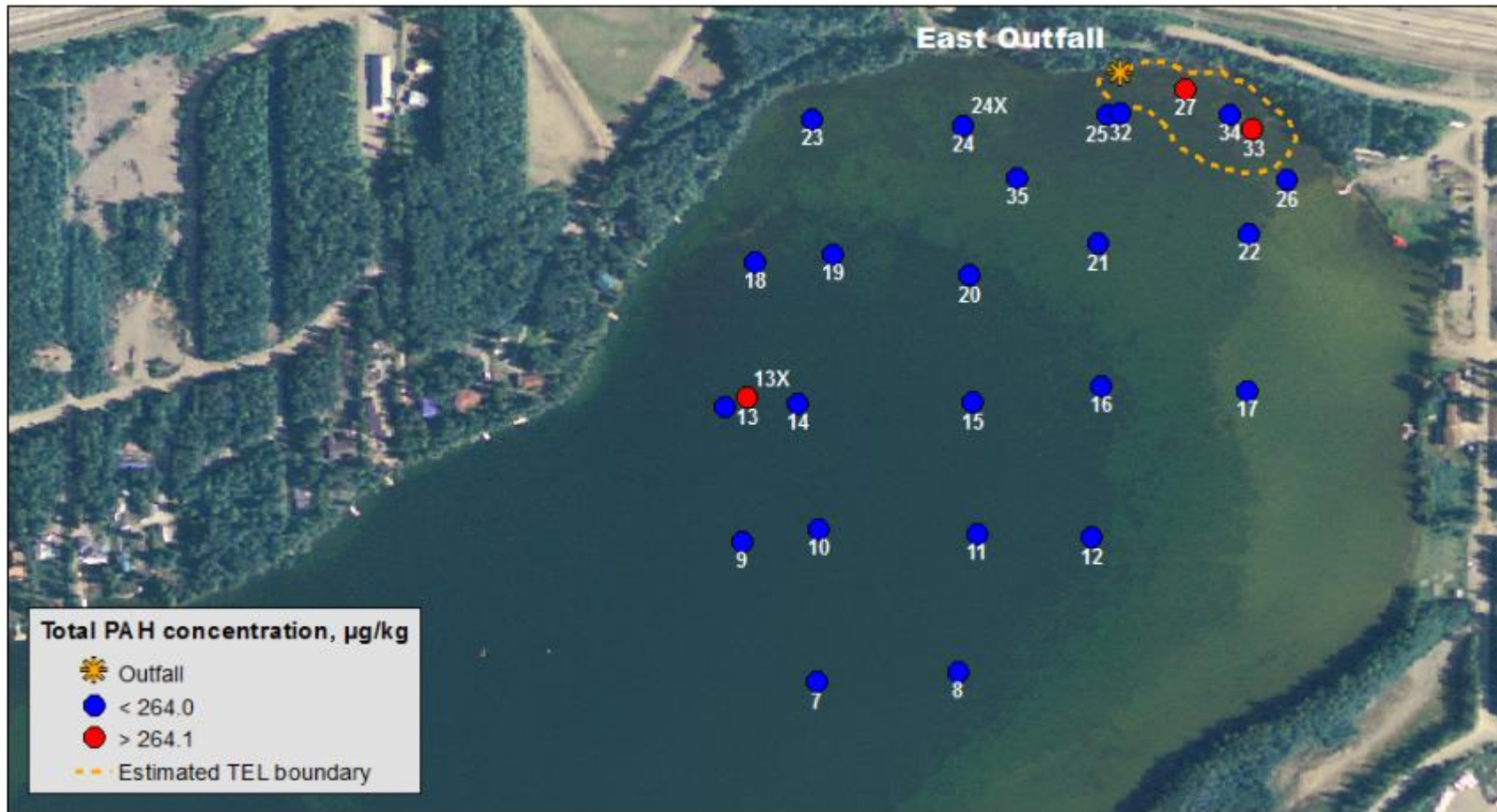
Figure 10. Distribution of bed sediment PAH concentrations adjacent to the east outfall. Red markers indicate sites where concentrations exceed TEL values. Dashed line is estimated area where PAH concentrations are likely to exceed TEL values.
