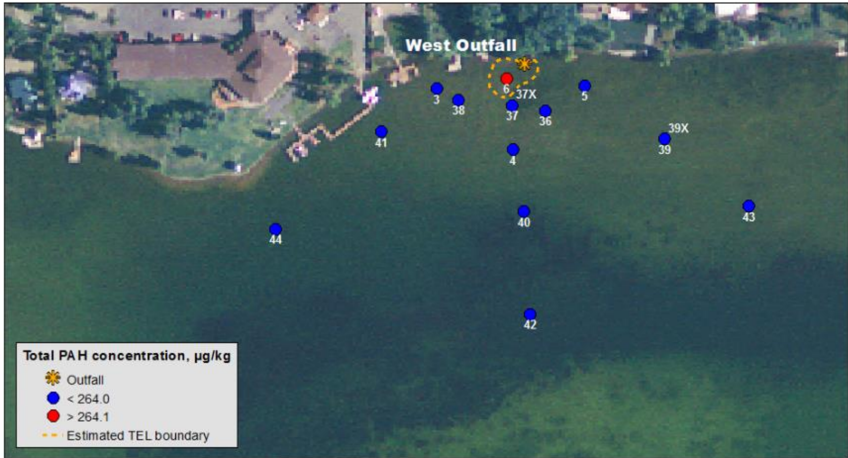
Figure 11. Distribution of bed sediment PAH concentrations adjacent to the west outfall. Red markers indicate sites where concentrations exceed TEL values. Dashed line is estimated area where PAH concentrations are likely to exceed TEL values.
