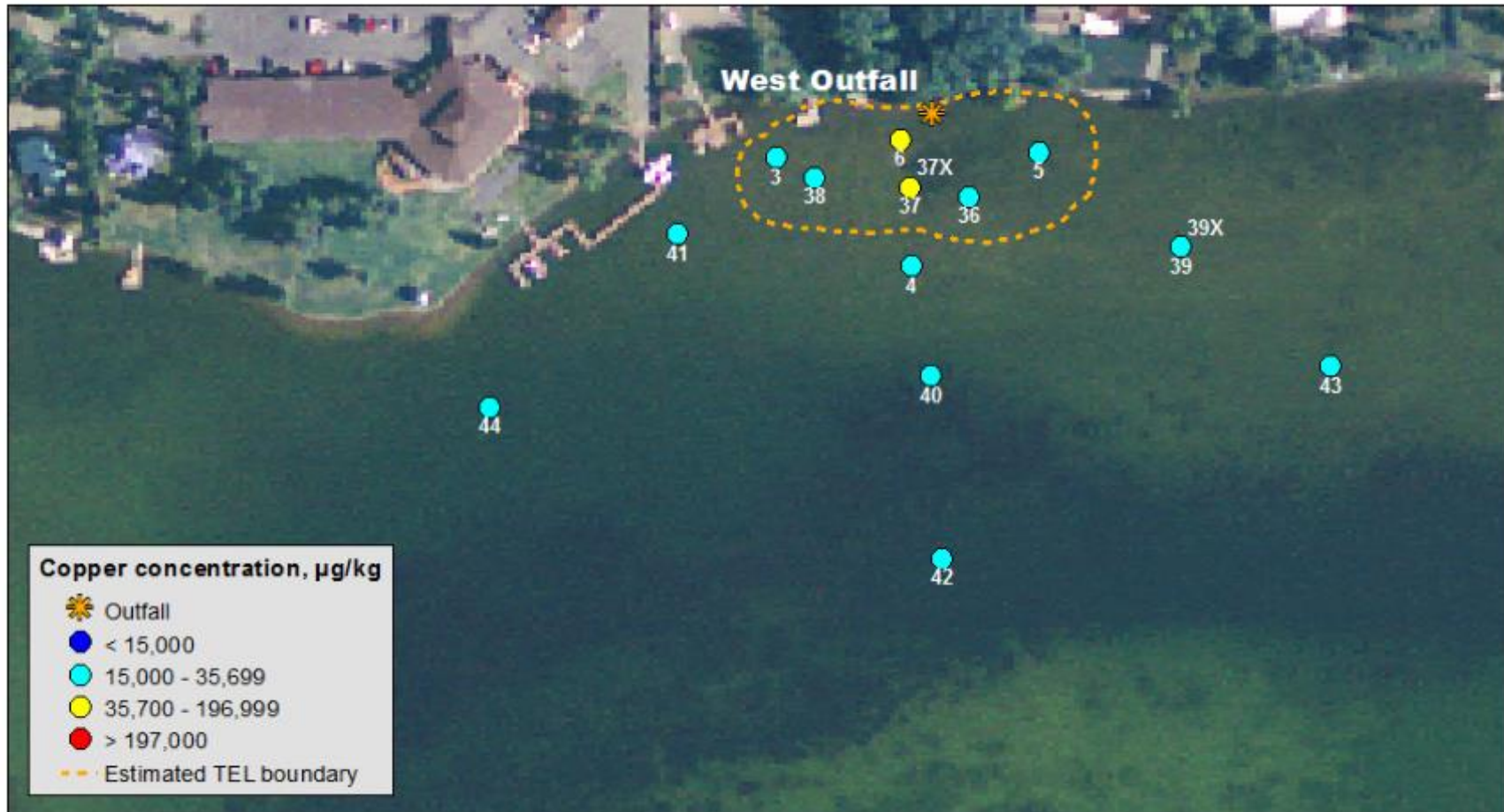
Figure 5. Distribution of bed sediment copper concentrations adjacent to the west outfall. Yellow markers indicate sites where concentrations exceed TEL values and red markers indicate sites that exceed PEL values. Dashed line is estimated area where copper concentrations are likely to exceed TEL values.
