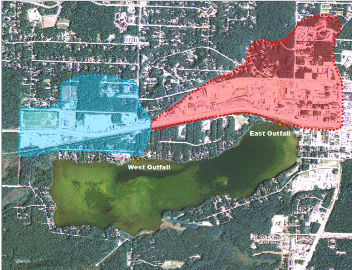
Figure 1. Aerial photograph of Lucile Lake and surrounding area showing estimated drainage area for east (309 acres) and west outfalls (212 acres).
