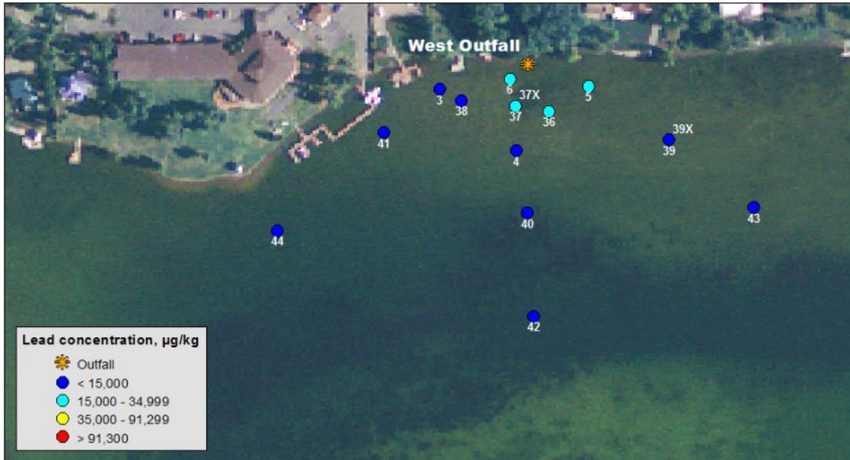
Figure 9. Distribution of bed sediment lead concentrations adjacent to the west outfall.
