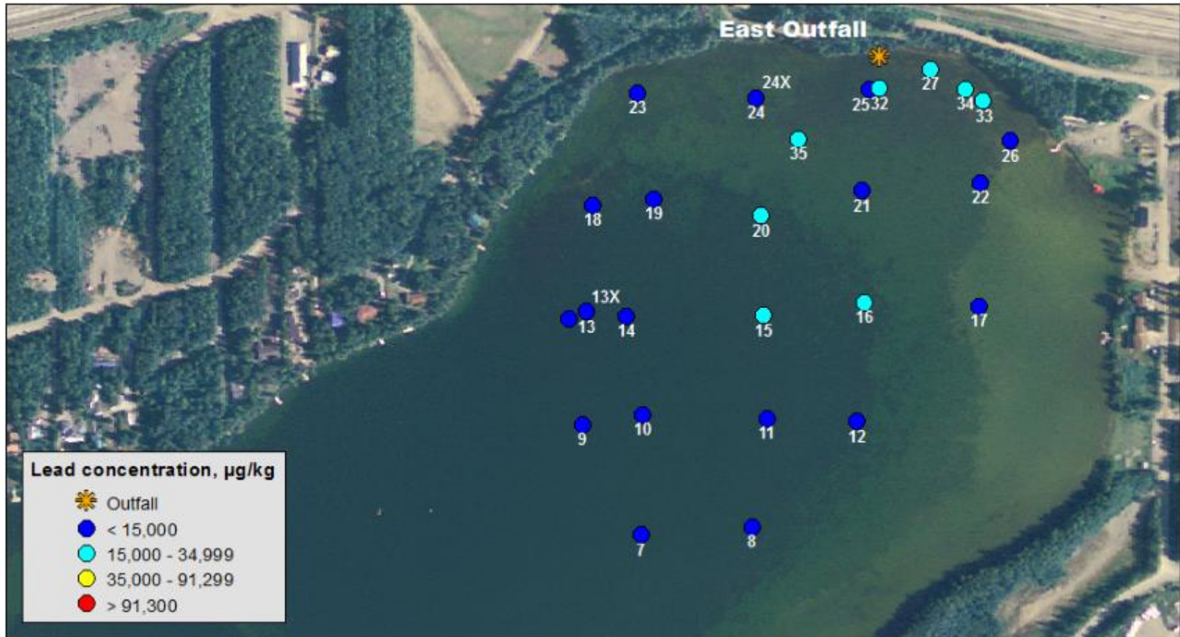
Figure 8. Distribution of lead sediment concentrations adjacent to the east outfall.
