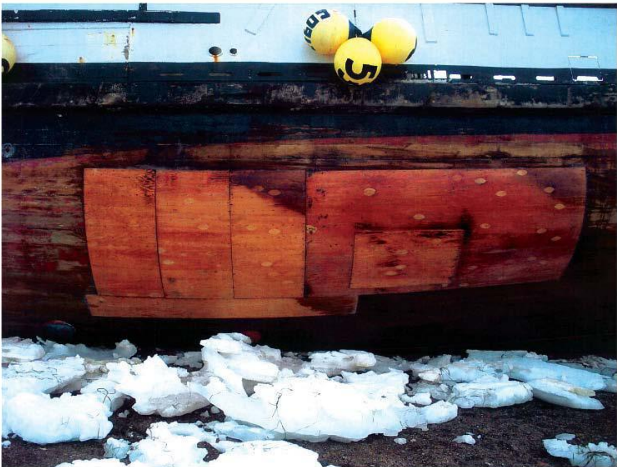
Photo taken by RP representative showing temporary repairs to hull of F/V Kupreanof.
