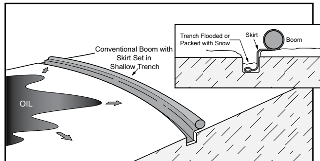
Figure PTS-7. Trench deployment using boom to enhance the oil barrier.
