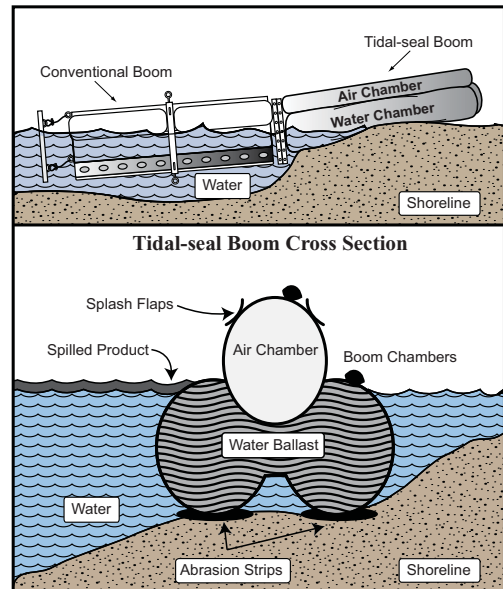
Figure DV-4. Tidal-seal boom configuration.
