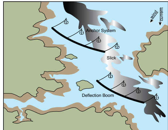
Figure DF-4. Deflection booming, fixed cascaded array.
