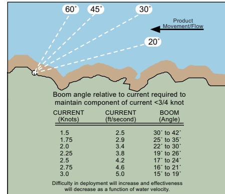
Figure DF-1. Boom angle relative to current.
