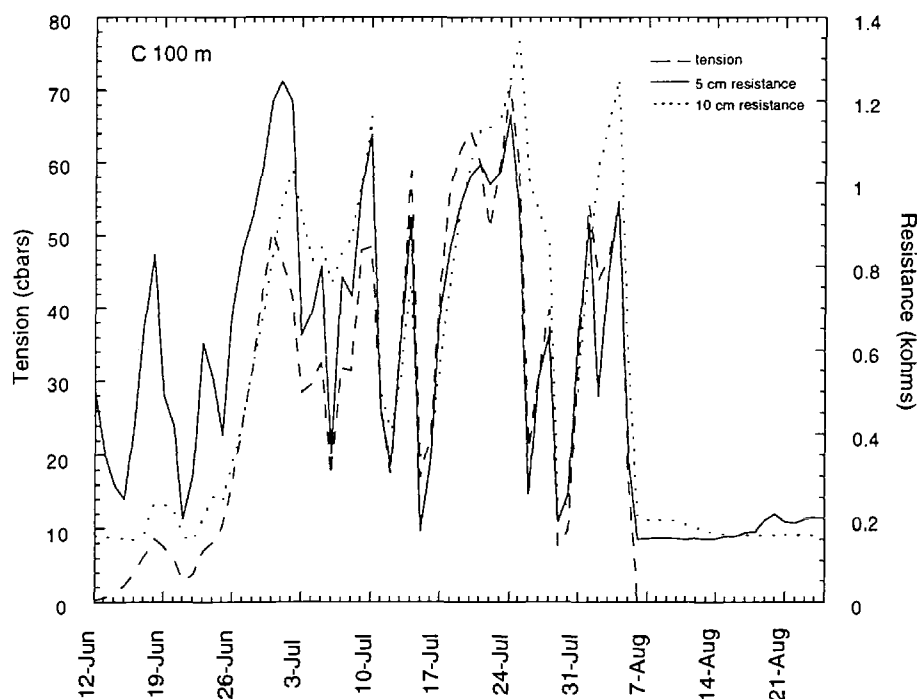
Figure III-2-12. Output from moisture sensors during summer of 1998. Increases in resistance and tension indicate drying.
