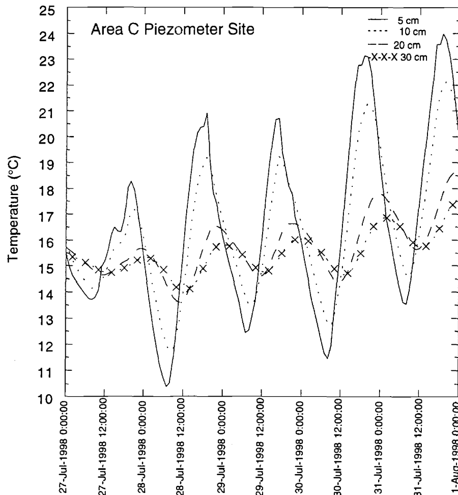
Figure III-2-17. Output from temperature sensors in Area C showing magnitude of sediment temperature fluctuations with depth.
