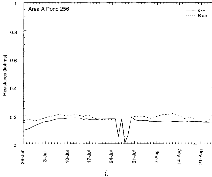
Figure III-2-12 (cont'd). Output from moisture sensors during summer of 1998. Increases in resistance and tension indicate drying.
