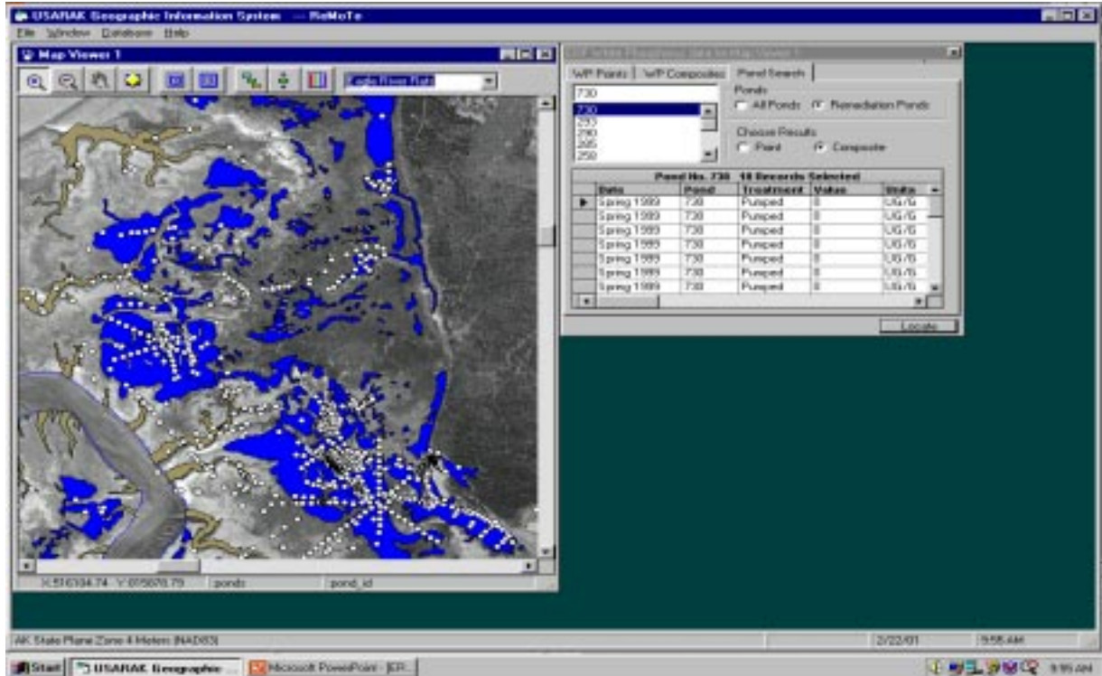
Figure IV-1-1. Example of a screen from the USARAK GIS database for contaminants showing all point and composite sediment samples analyzed for white phosphorus. The database permits the user to locate and obtain all of the point or composite samples collected and analyzed for any pond. Here the composite samples collected in pond 730 are listed. It is necessary to scroll down to see all of the samples and the concentrations.
