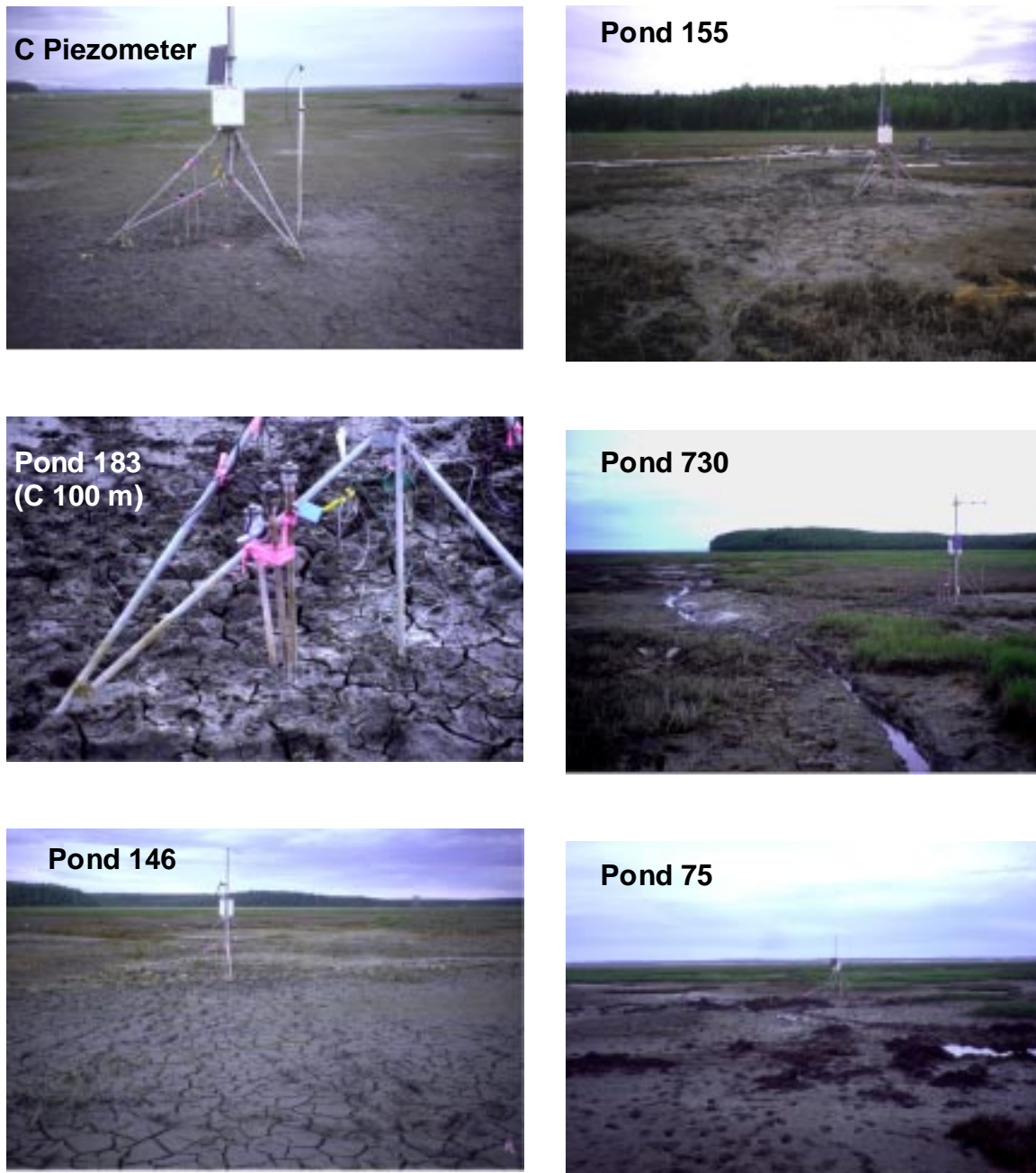
Figure III-2-8. Datalogger station photographed near peak drying conditions in June 2000.
