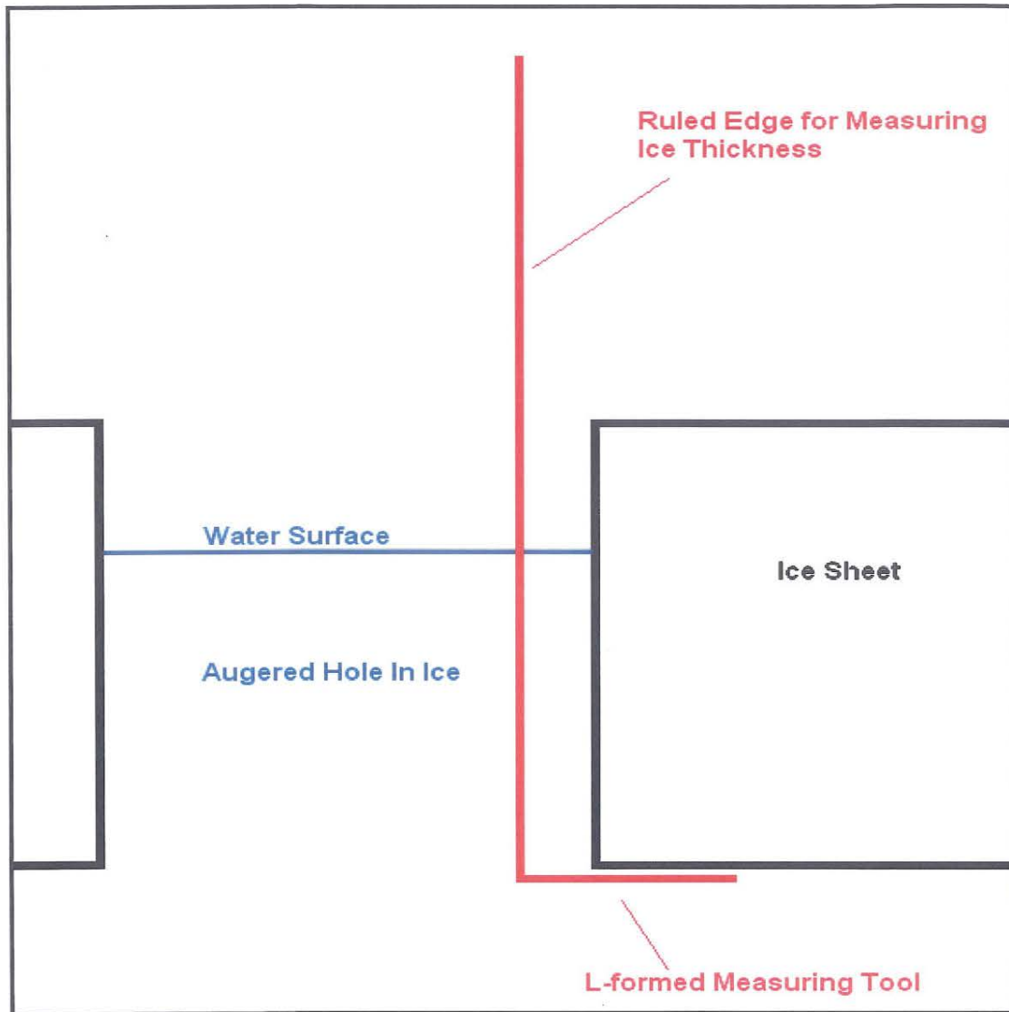
Figure 2: Diagram of L-shaped measuring tool and ice thickness measurement scenario
