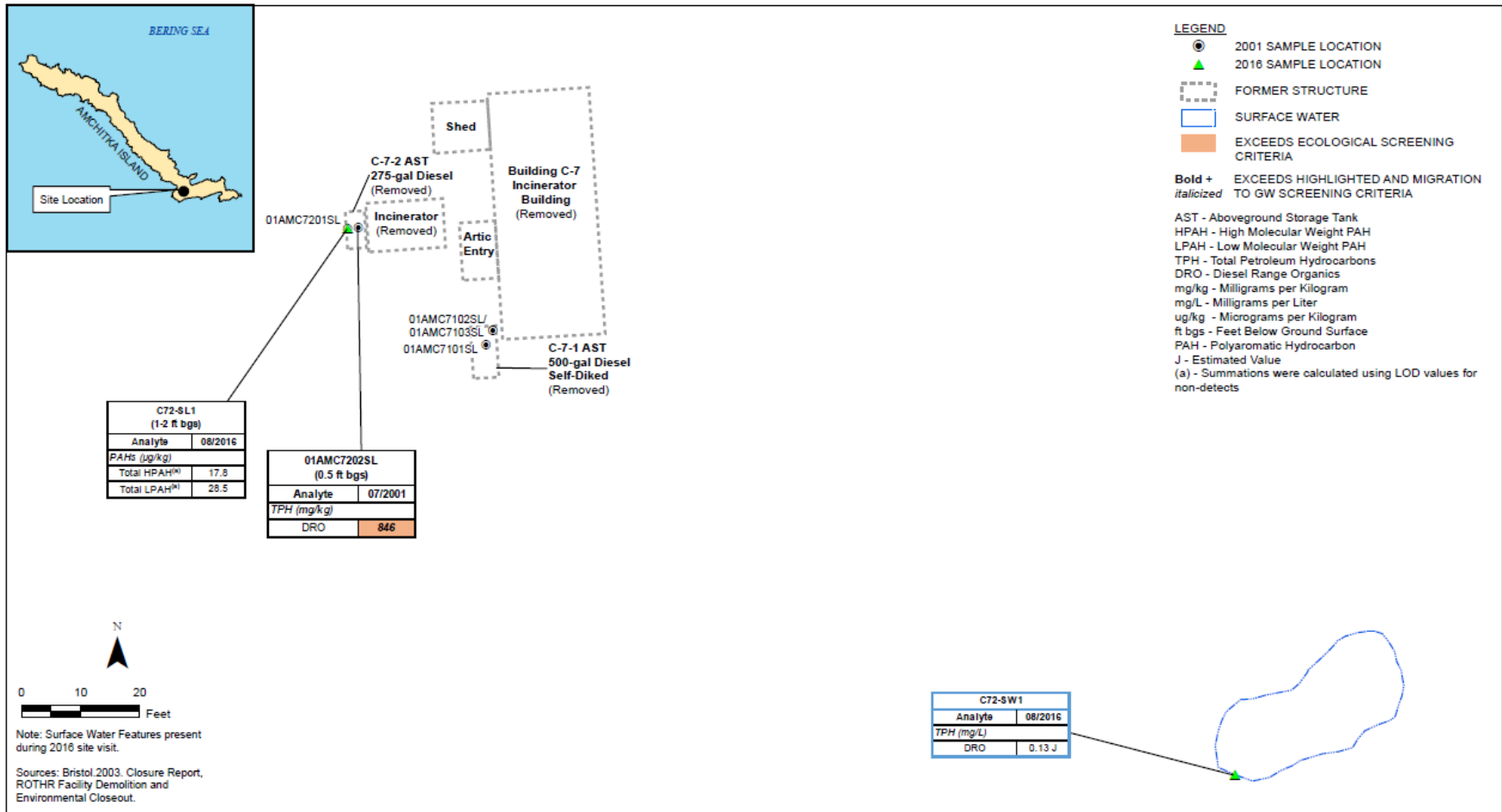
Figure 4-59. AST C-7-1 and AST C-7-2 Detections and Comparison to Screening Criteria
