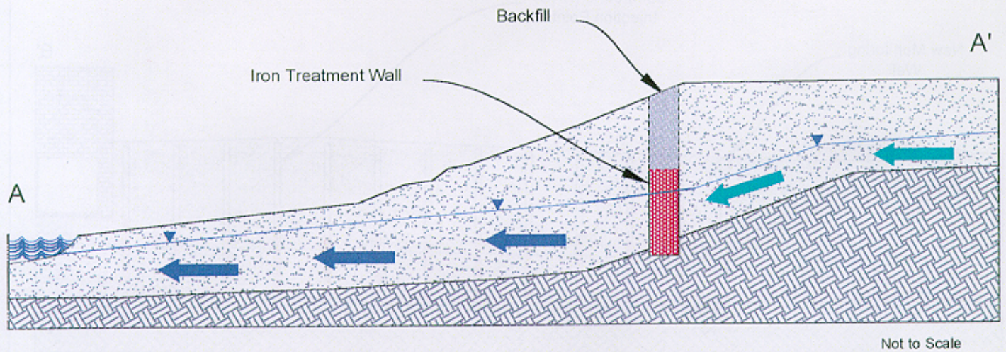
Figure 5 Conceptual Drawing: Contingent Remedial Alternative for Lower Plume Area
