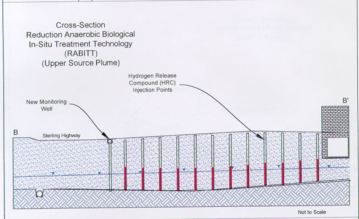
Figure 6 Conceptual Drawing: Preferred Remedial Alternative for Upper Plume Area
