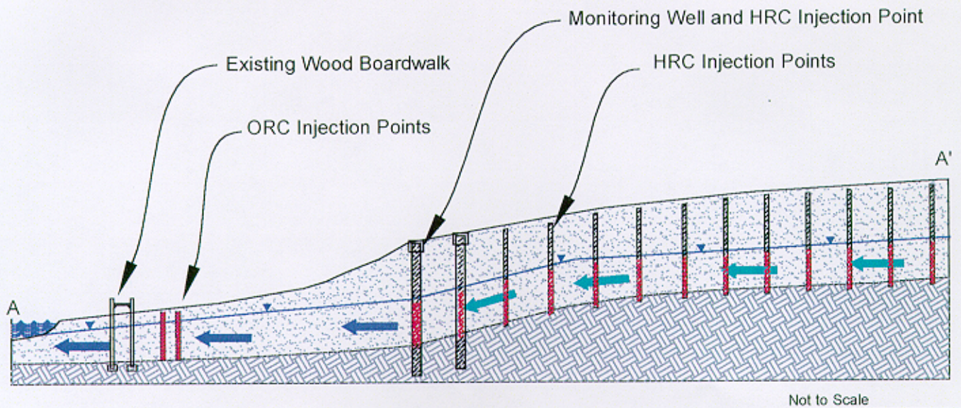
Figure 4 Conceptual Drawing: Preferred Remedial Alternative for Lower Plume Area
