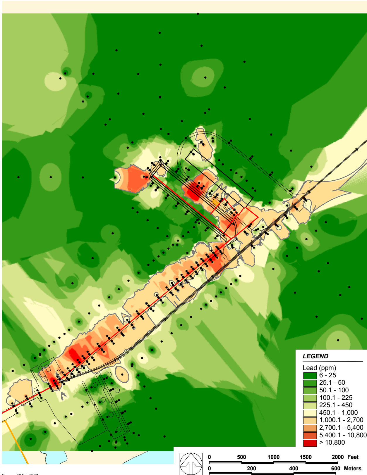
Figure 2. Contour map of lead concentrations in 1996
