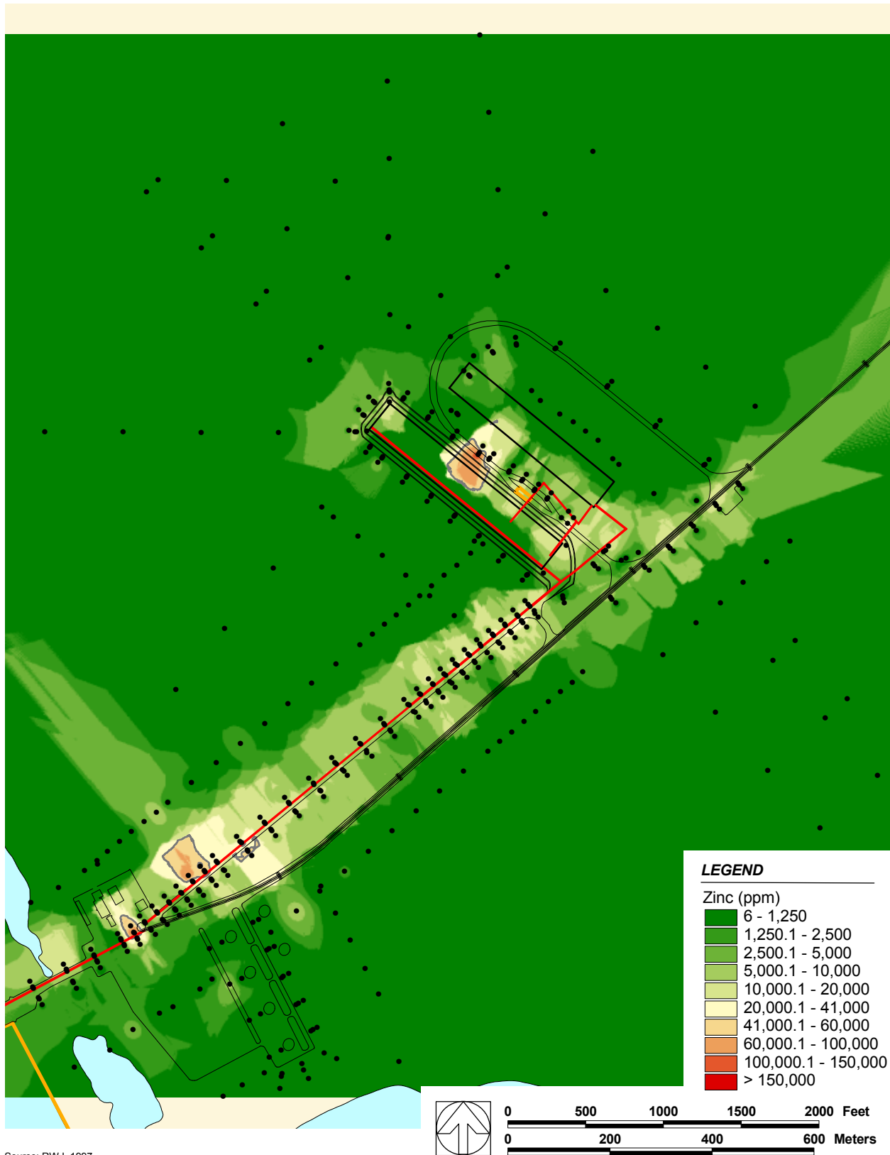
Figure 3. Contour map of zinc concentrations in 1996
