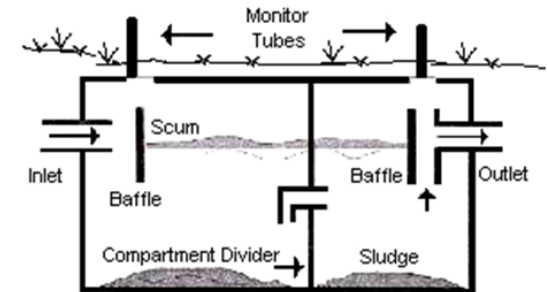
Scum layer is made of floating oils and greases. Sludge layer is made of heavier solids.
