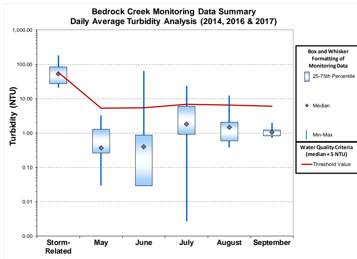
Figure 2-5. TMDL threshold values based on average daily turbidity measurements at Bedrock Creek
