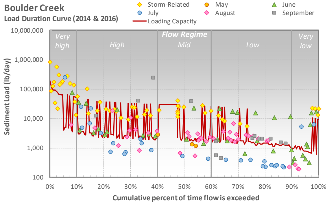
Figure 5-2. Allowable and existing sediment loads as a function of flow in the Boulder Creek subwatershed
