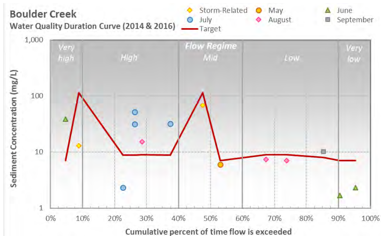
Figure 3-19. TSS values for Boulder Creek as a function of flow (2014 & 2016)
