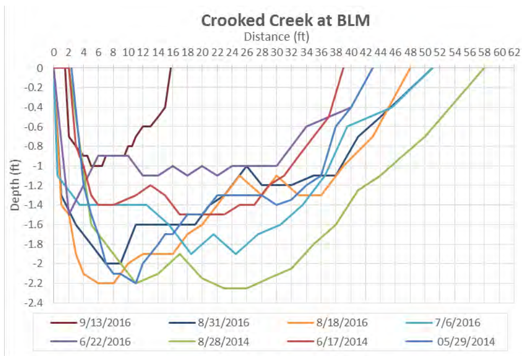
Figure 3-6. Cross-section data at Crooked Creek monitoring station
