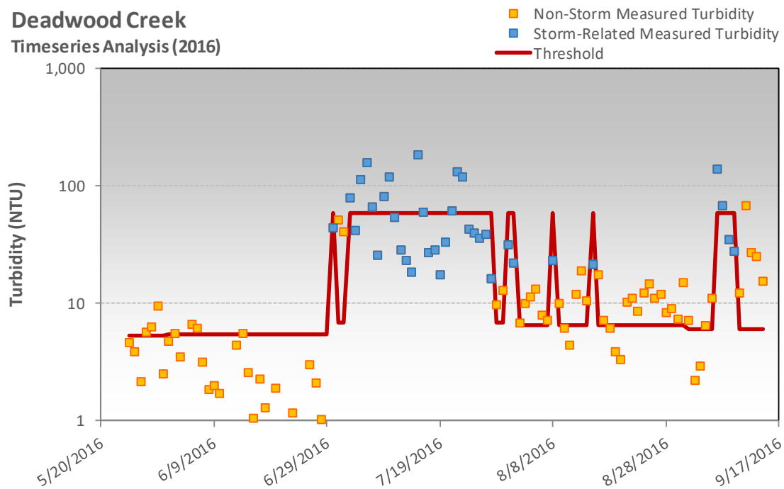
Figure A-10. Measured turbidity time series analysis for Deadwood Creek (2016)
