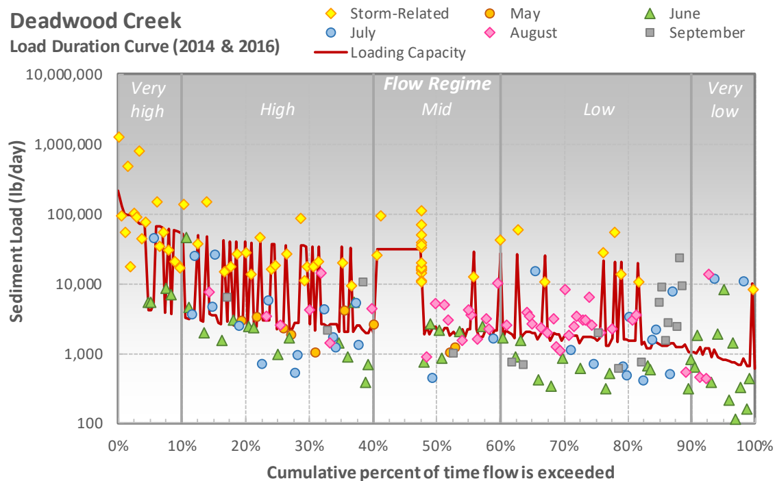
Figure 5-3. Allowable and existing sediment loads as a function of flow in the Deadwood Creek subwatershed
