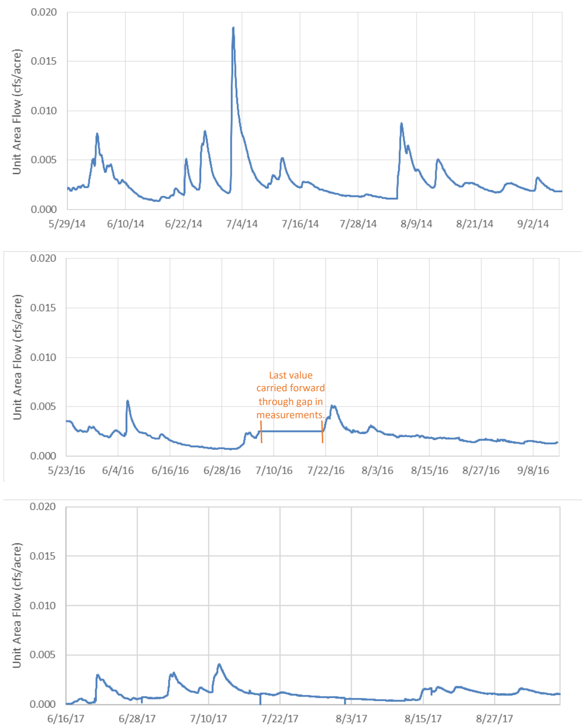
Figure 3-13. Estimated unit area flows at Crooked Creek at BLM (2014, 2016 and 2017)
