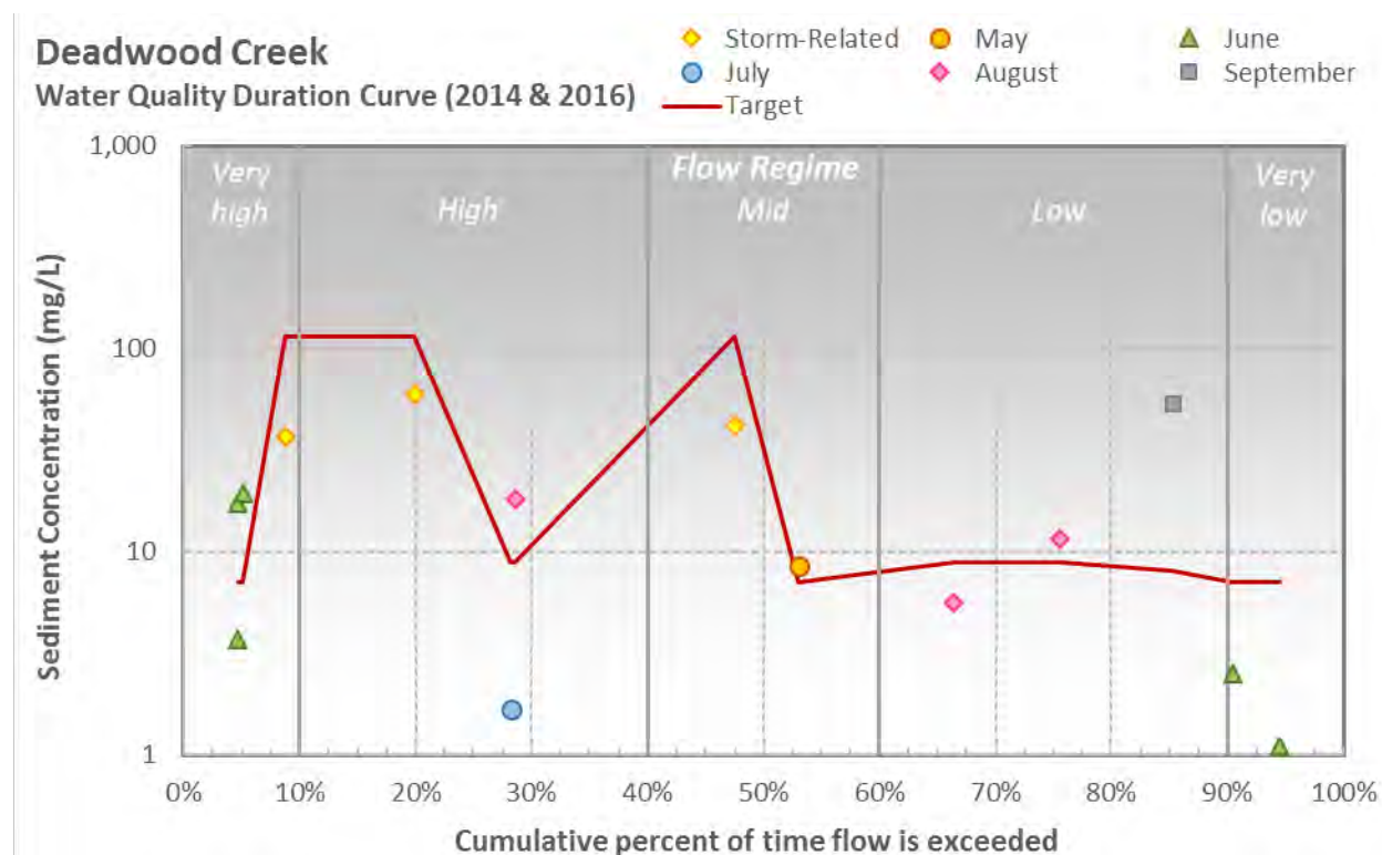
Figure 3-20. TSS values for Deadwood Creek as a function of flow (2014 & 2016)
