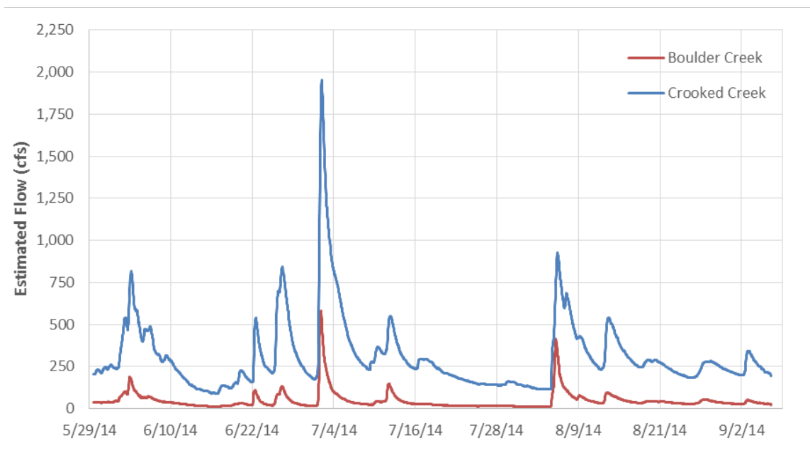
Figure 3-10. Estimated 2014 flows for Boulder and Crooked creeks
