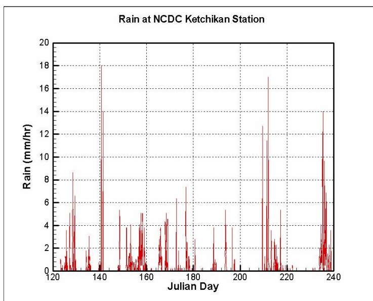
Figure B-5. Rain registered at NCDC Ketchikan station.
