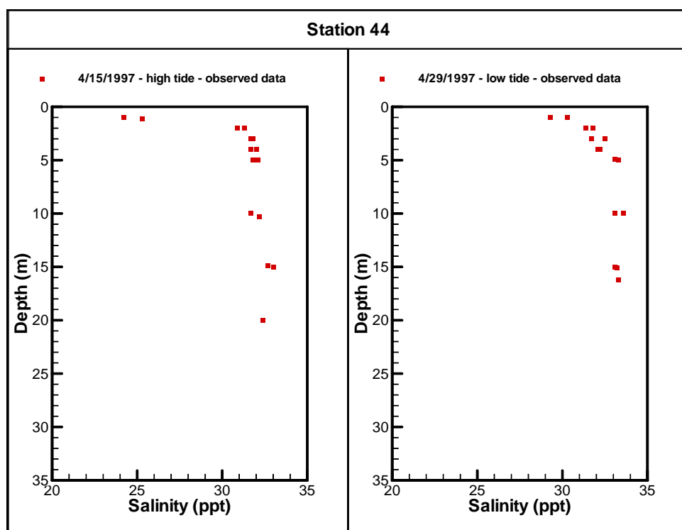
Figure C-16. Salinity profiles at Station 44 measured in April 1997
