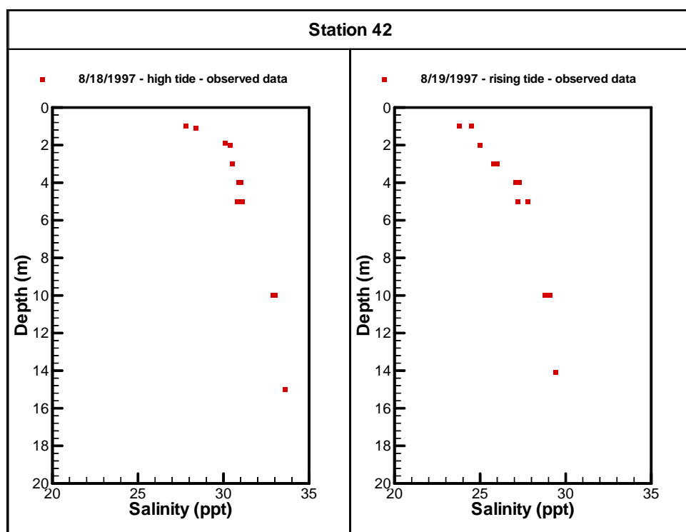
Figure C-10. Salinity profiles at Station 42 measured in August 1997
