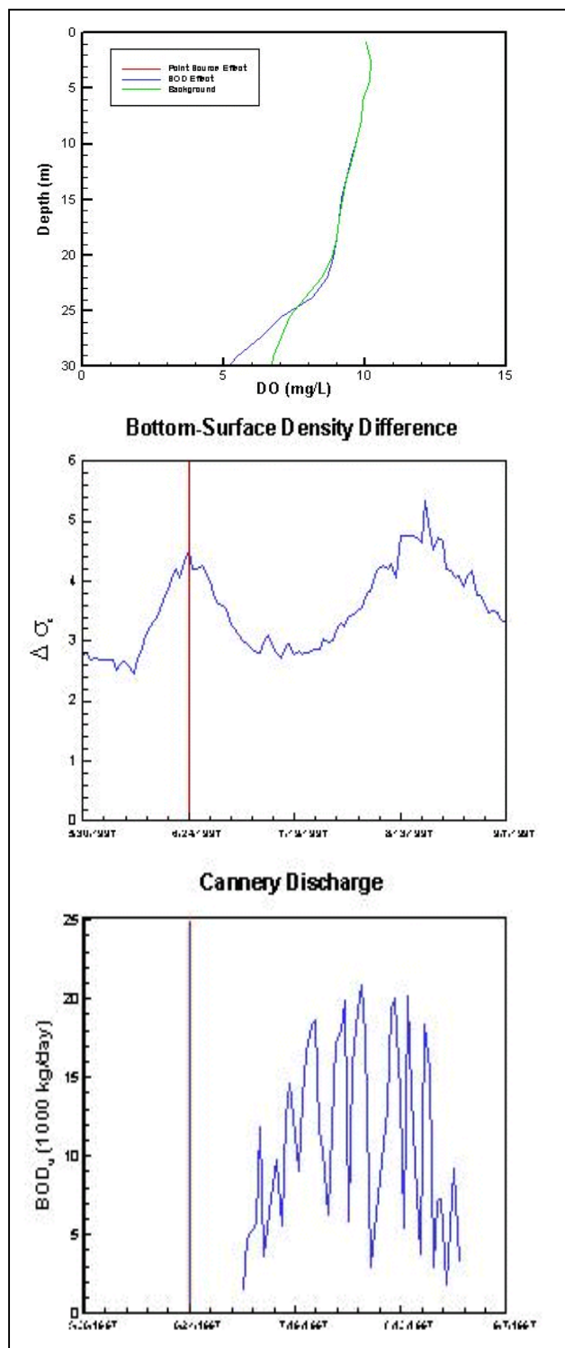
Figure B-24. Simulated dissolved oxygen profile, vertical density difference, and WPC discharge on June 24, 1997 at Station 44.
