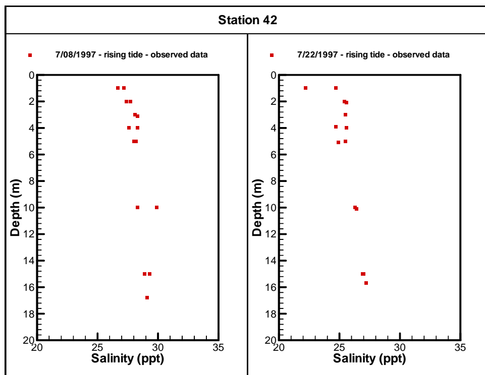
Figure C-9. Salinity profiles at Station 42 measured in July 1997
