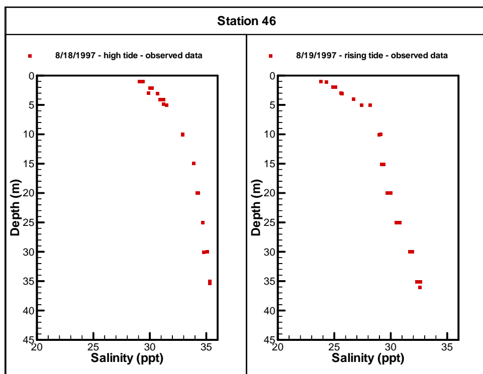
Figure C-30. Salinity profiles at Station 46 measured in August 1997
