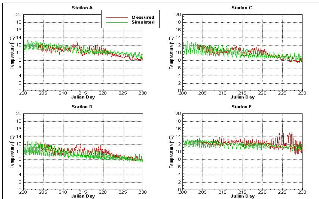
Figure B-11. Comparisons of temperature time series at Stations A through E.
