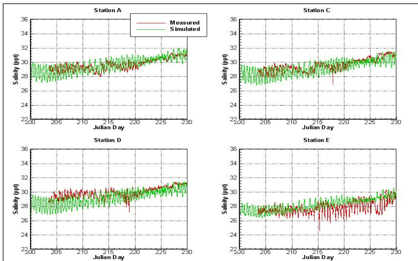
Figure B-10. Comparisons of salinity time series at Stations A through E.
