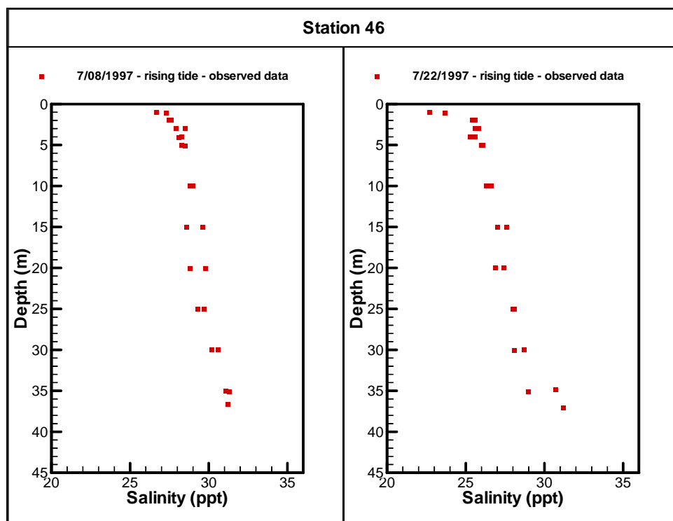
Figure C-29. Salinity profiles at Station 46 measured in July 1997
