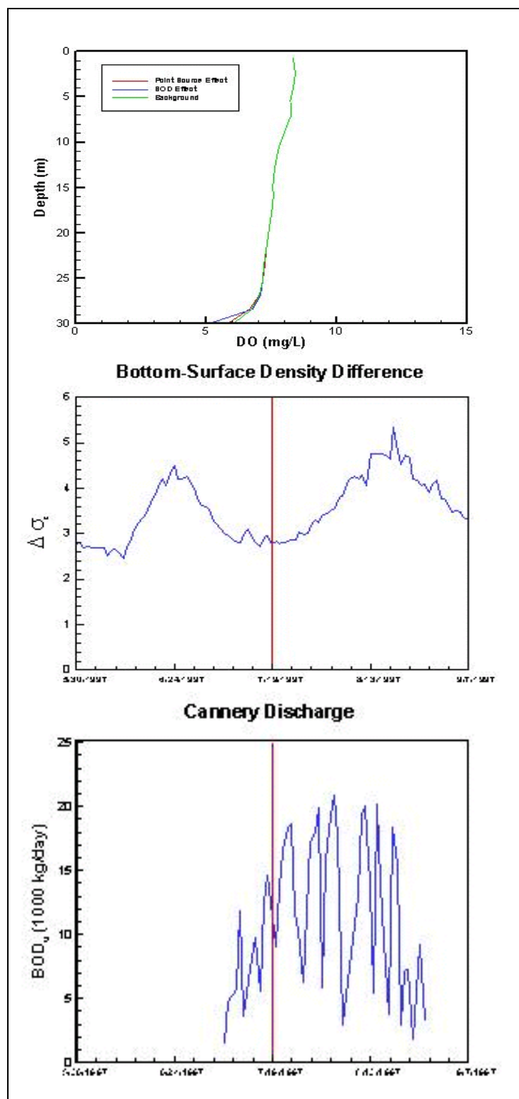
Figure B-25. Simulated dissolved oxygen profile, vertical density difference, and WCPC discharge on July 19, 1997 at Station 44.
