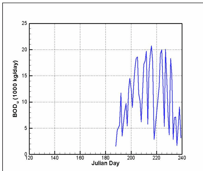
Figure B-20. CBOD u load from WPCPC facility.
