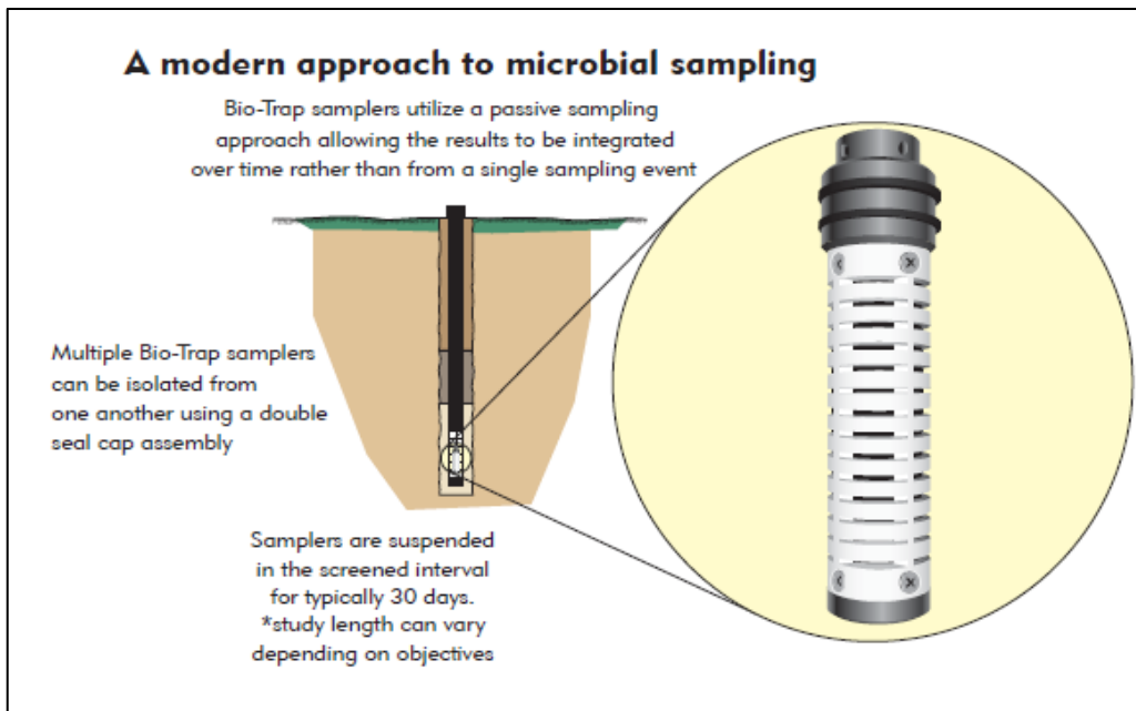
Figure 20. Bio-Trap™ passive microbial sampling device (Figure courtesy Microbial Insights, Inc., Knoxville TN)
