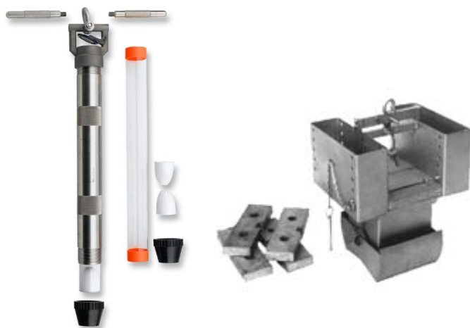
Figure 24. a) Sediment hand core sampler; b) box corer (image sources: a) Forestry Suppliers, Inc.; b) Wildco)
