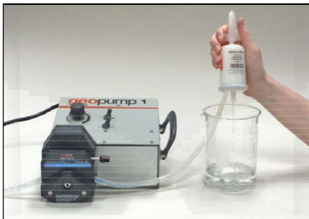
Figure 13. Geopump™ Peristaltic Pump. Photograph with permission from Geotech Environmental Equipment, Inc.
