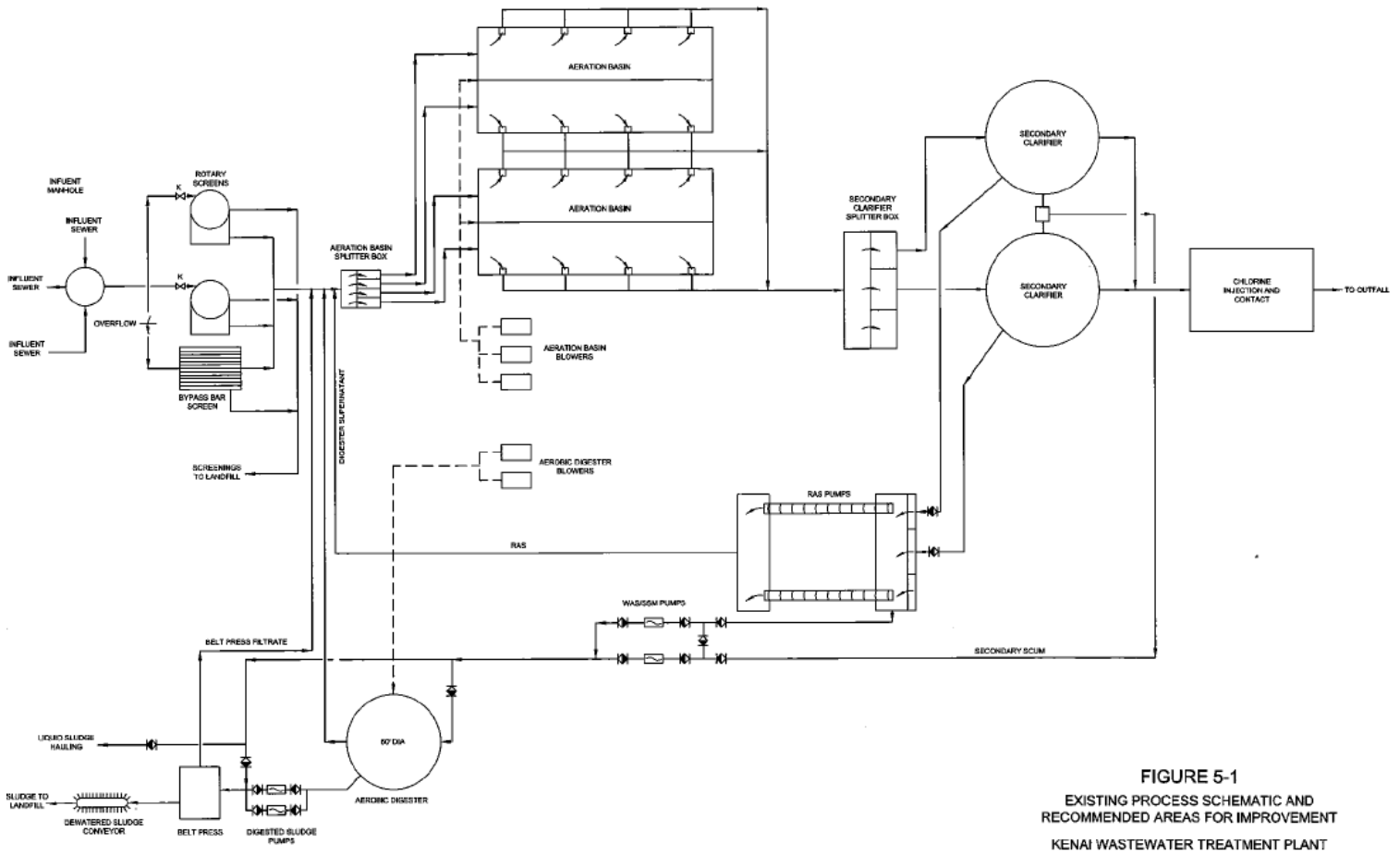
Figure 2: Kenai Wastewater Treatment Plant Process Flow Diagram
