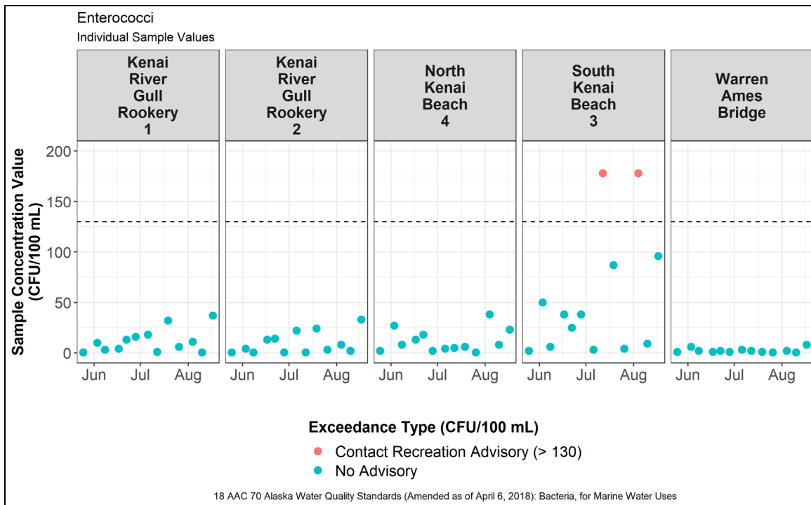
Figure 7 – Enterococci sample concentrations from lower Kenai River sites in 2020, color coded by exceedance standard criteria. Dotted lines indicates the criteria thresholds for individual samples of 130 CFU/100 mL.
