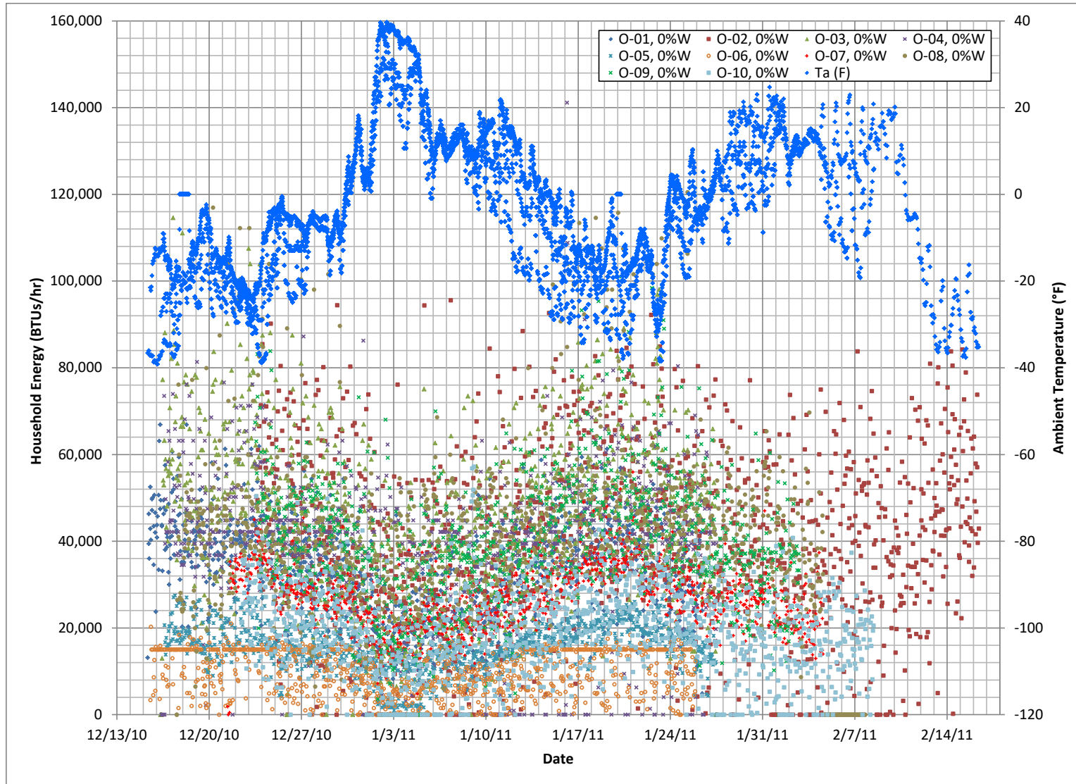
Figure 7-6-7 Hourly Instrumented Energy Usage (BTU/hour), Oil Only Households
