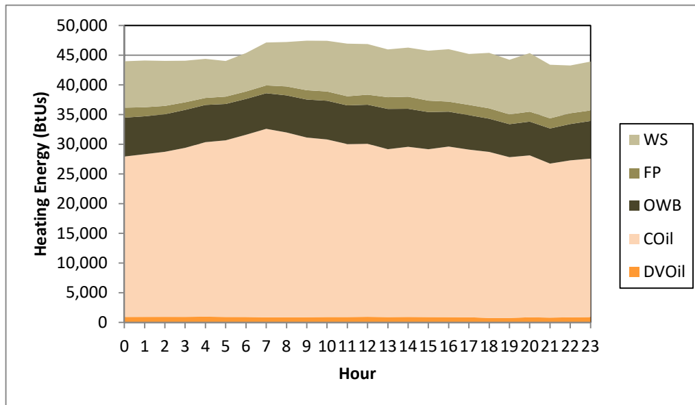
Figure 7-6-19 Combined Model Energy Use Case: Dwelling Size = 2,129 ft 2 , Temp = -20°F, Day Type = WD, WS=22%, FP=1%, OWB=10%, CentOil=64%, DVOil=3%
