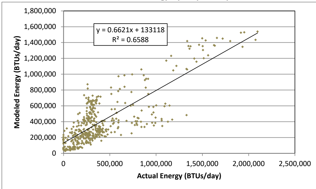
Figure 7-6-13 Modeled vs. Actual Household Energy by Day - Daily Wood Stove BTUs
