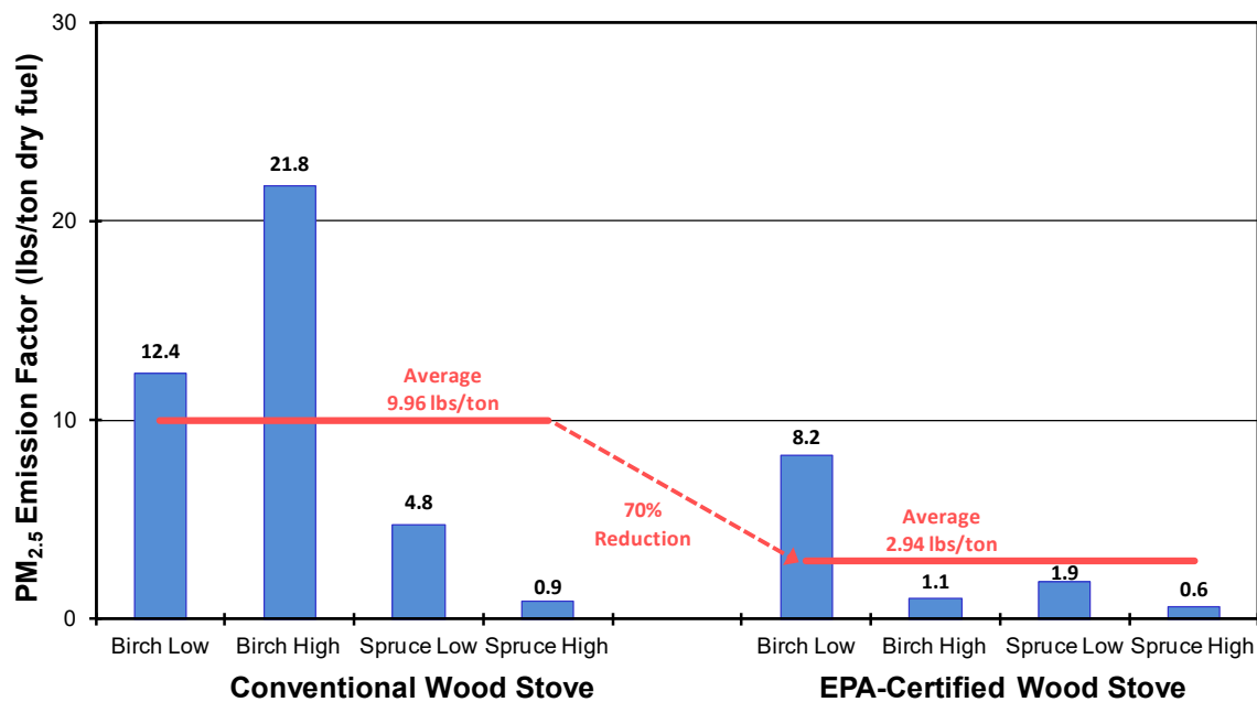
Figure 7-6-28 PM 2.5 Emission Factors from OMNI Testing for Conventional (left) & EPA-Certified (right) Wood Stoves by Wood Species and Firing Rate
