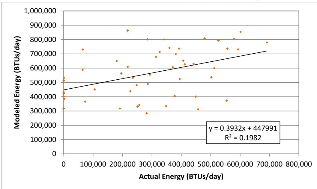
Figure 7-6-14 Modeled vs. Actual Household Energy by Day - Daily Fireplace BTUs
