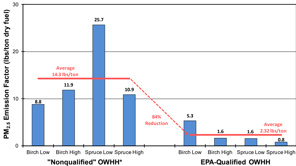
Figure 7-6-29 PM 2.5 Emission Factors from OMNI Testing for Non-Qualified (left) & EPA-Qualified (right) OWHHs by Wood Species and Firing Rate
