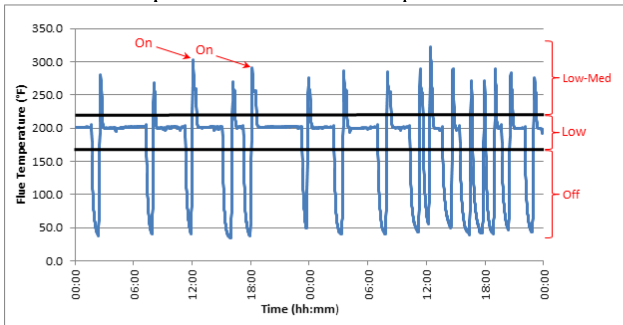
Figure 7-6-6 Sample Direct Vent Oil Heater Fuel Temperature Trace
