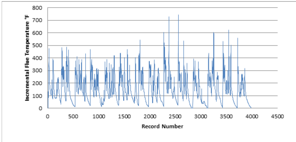
Figure 7-6-4 Example Wood Stove Fuel Temperature Trace, Household M-02
