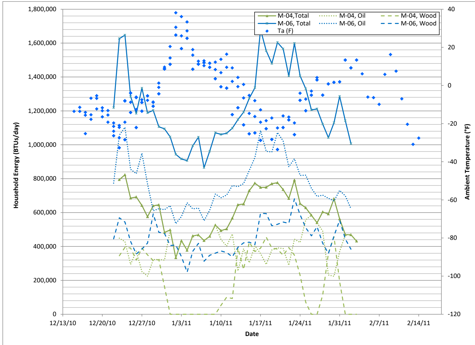
Figure 7-6-11 Daily Instrumented Energy Usage (BTU/day) by Fuel Type, Mixed Households M-04 and M-06
