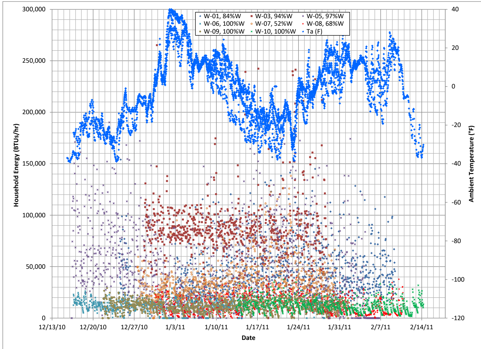
Figure 7-6-8 Hourly Instrumented Energy Usage (BTU/hour), Primary Wood Households
