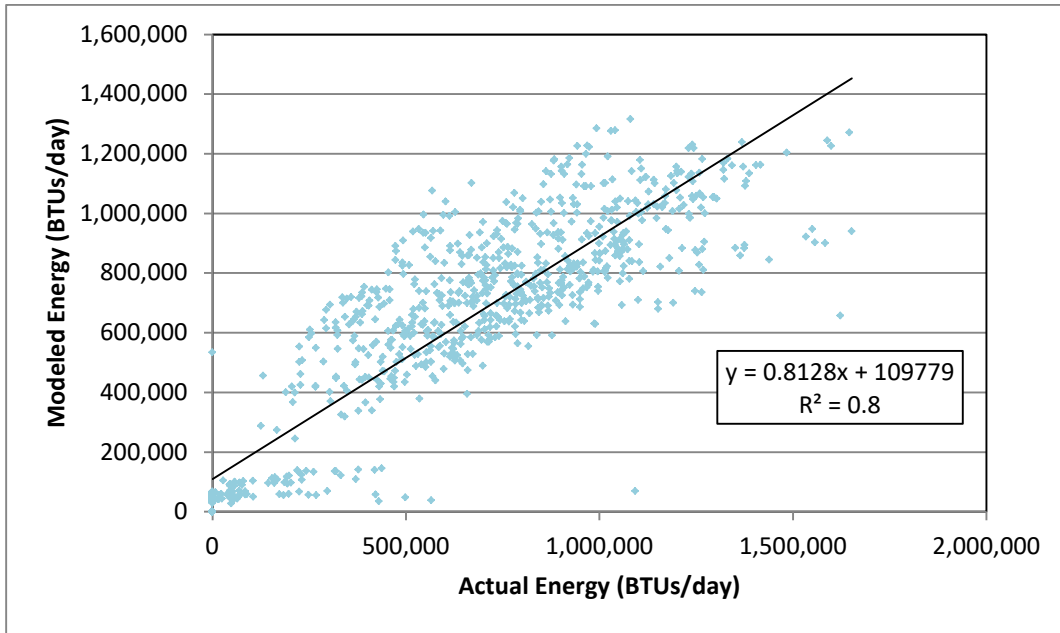
Figure 7-6-16 Modeled vs. Actual Household Energy by Day - Daily Central Oil Device BTUs
