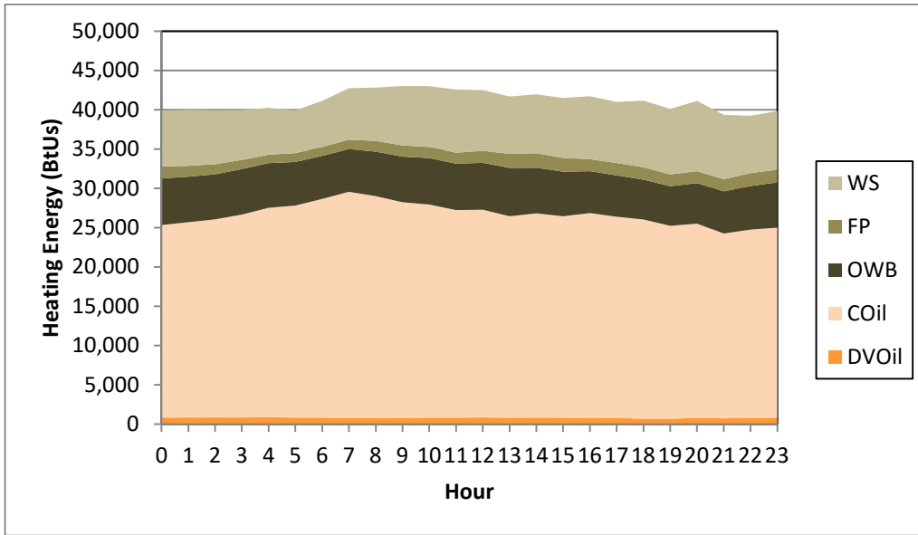
Figure 7-6-21 Combined Model Energy Use Case: Dwelling Size 1,500 ft 2 , Temp = -20°F, Day Type = WD, WS=22%, FP=1%, OWB=10%, CentOil=64%, DVOil=3%
