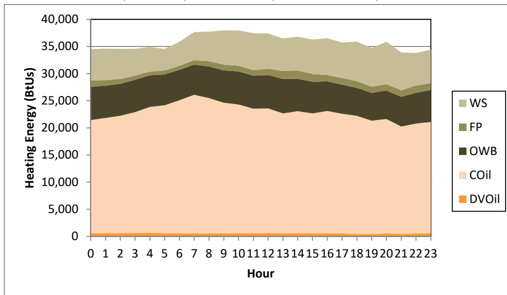
Figure 7-6-18 Combined Model Energy Use Case: Dwelling Size = 2,129 ft 2 , Temp = 0°F, Day Type = WD, WS=22%, FP=1%, OWB=10%, CentOil=64%, DVOil=3%
