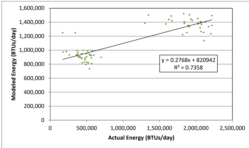
Figure 7-6-15 Modeled vs. Actual Household Energy by Day - Daily Outdoor Wood Boiler BTUs
