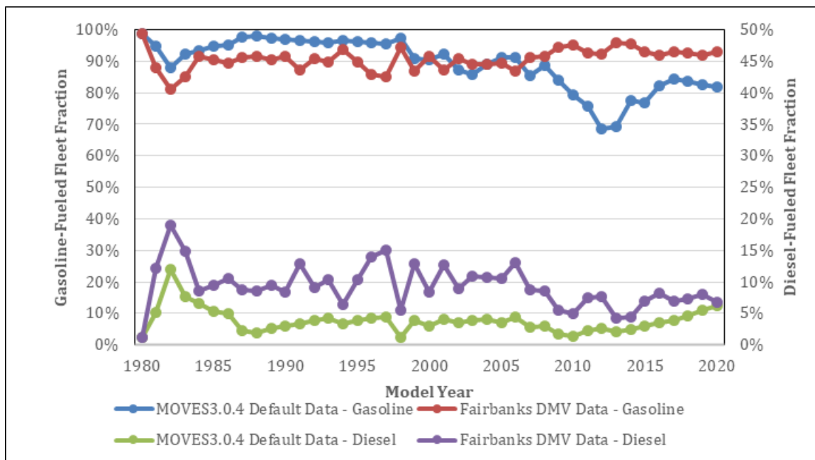
Figure 7-6-33 Comparison of Passenger Truck Gasoline-and Diesel Fuel Vehicle Fractions by Model Year Fairbanks DMV Data vs. MOVES3 Defaults
