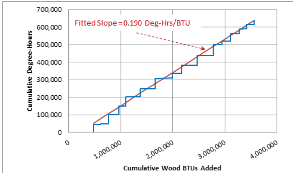
Figure 7-6-5 Cumulative Wood Stove BTUs and Flue Degrees, Household M-02
