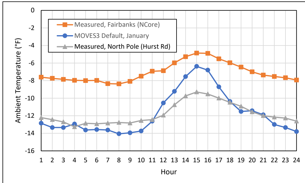
Figure 7-6-34 Comparison of MOVES Default and Measured Average Diurnal Temperature Profiles
