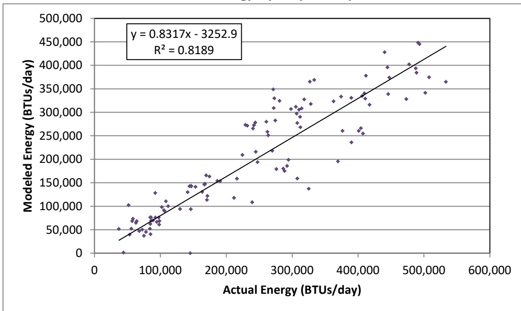
Figure 7-6-17 Modeled vs. Actual Household Energy by Day - Daily Direct Vent Heater BTUs
