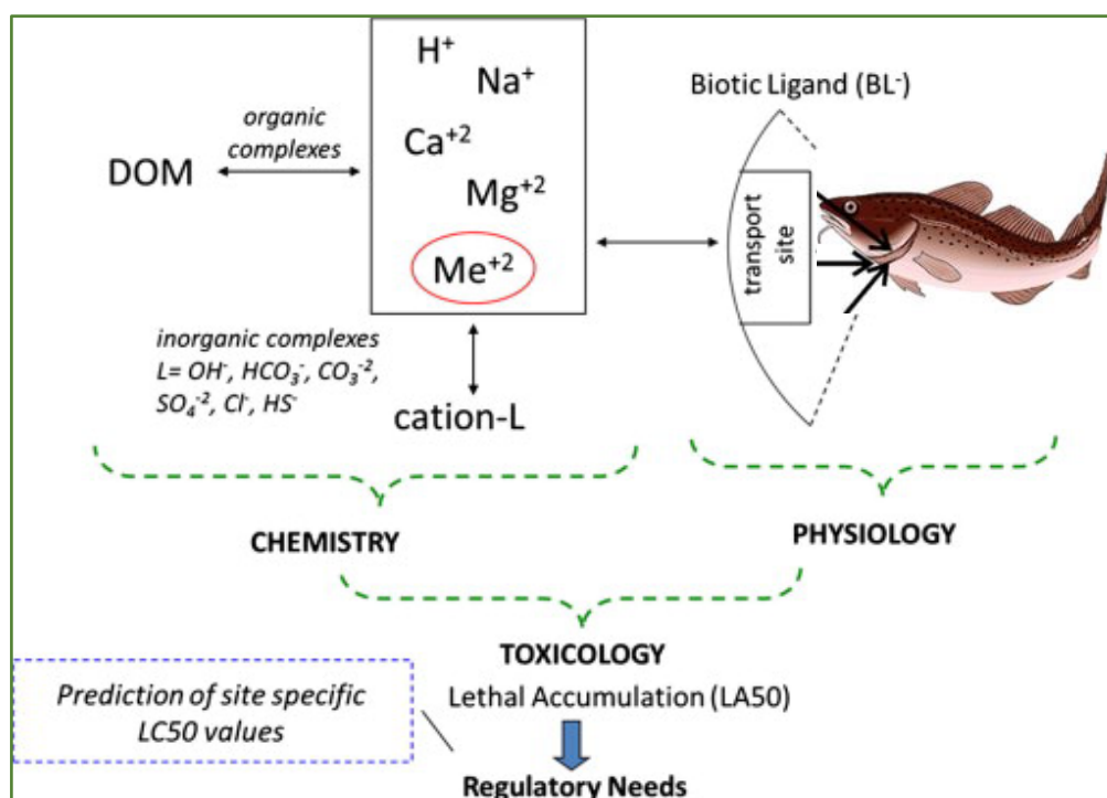
Figure 1: Schematic of the Biotic Ligand Model (Smith, Balistrieri, Todd, 2015)
