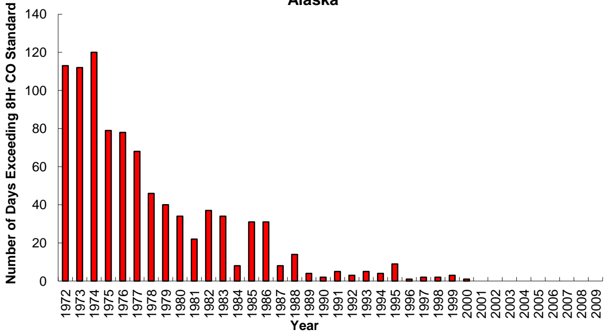
Number of Days Exceeding the 8-Hour CO Standard - Fairbanks, Alaska
