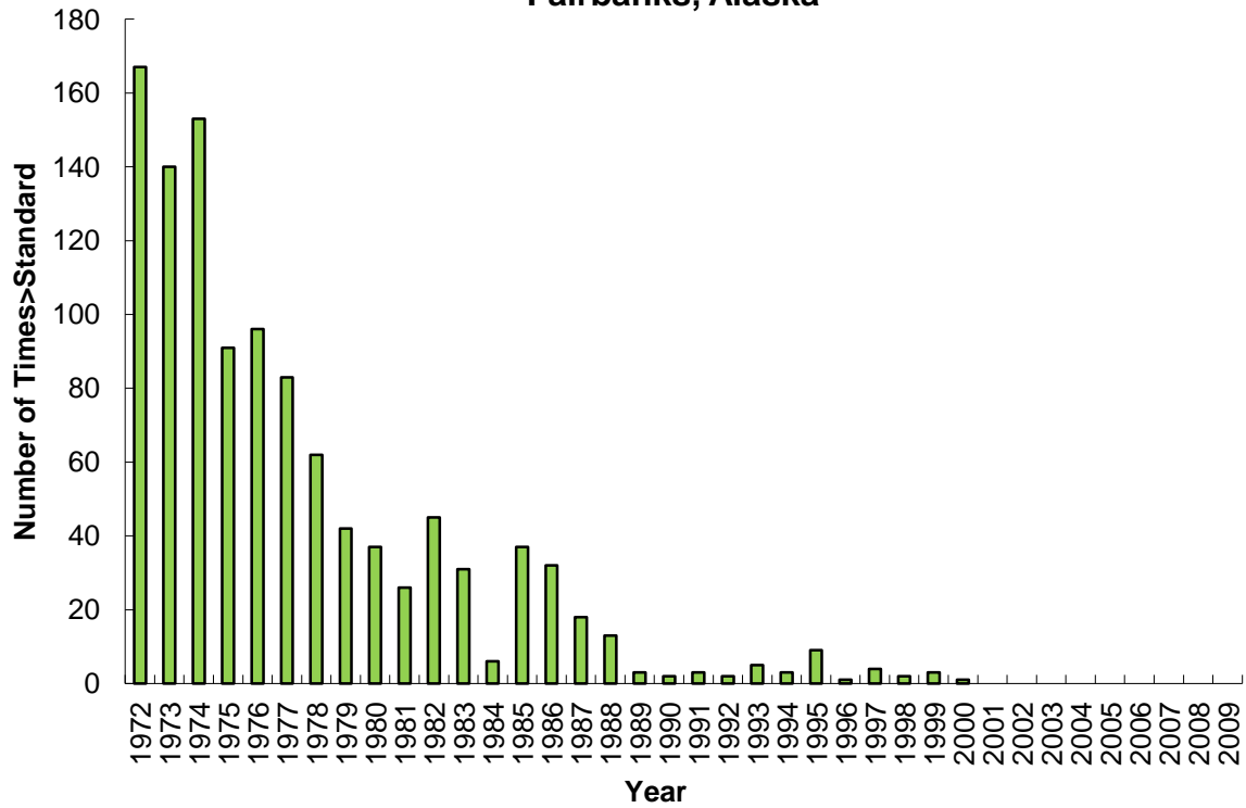
Number of Times the 8-Hour CO Health Standard was Exceeded Fairbanks, Alaska
