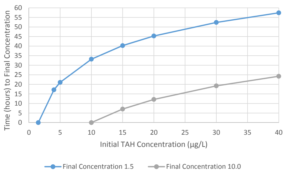
Figure 16. Time required for TAH concentrations to decline to final concentrations of 1.5 \mu\text{g/L} (blue line) or 10 \mu\text{g/L} (grey line).
