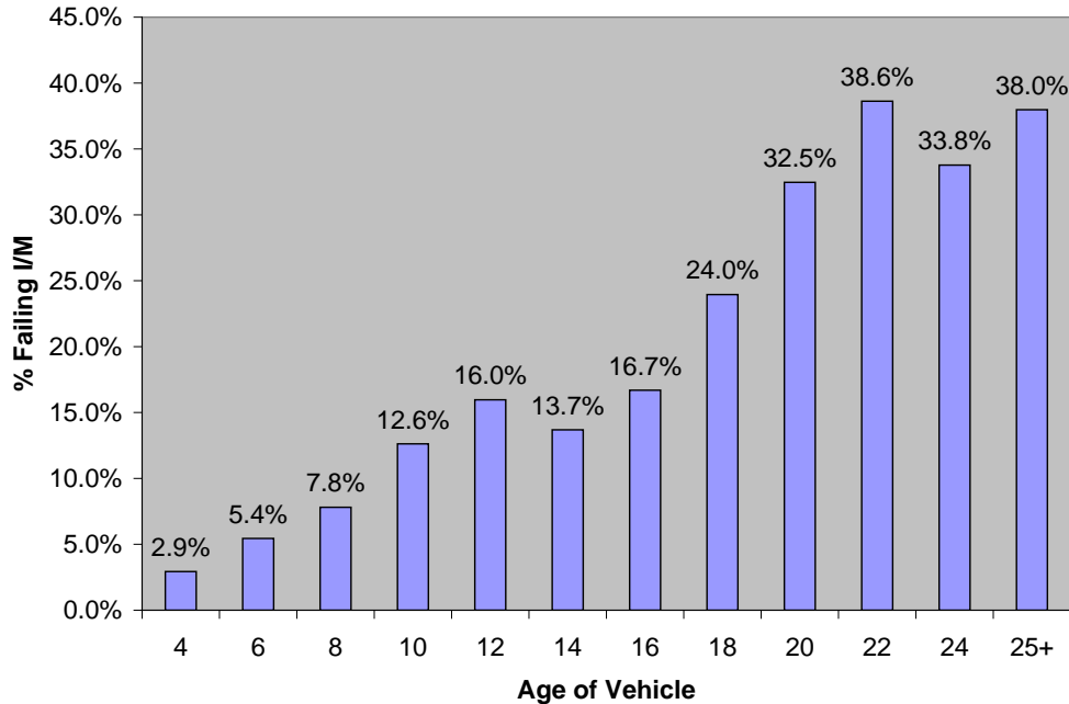
Figure III.B.5-1 I/M Fail Rate vs. Vehicle Age in 2006
